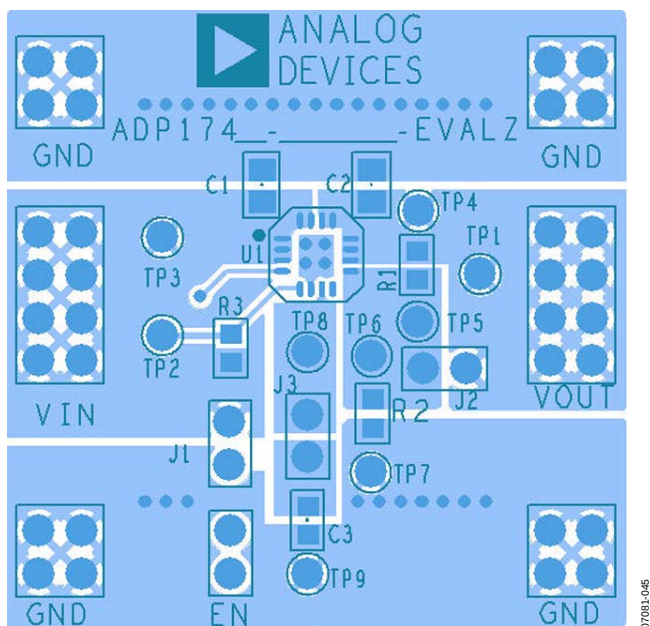
Figure 47. Typical Board Layout, Top Side
