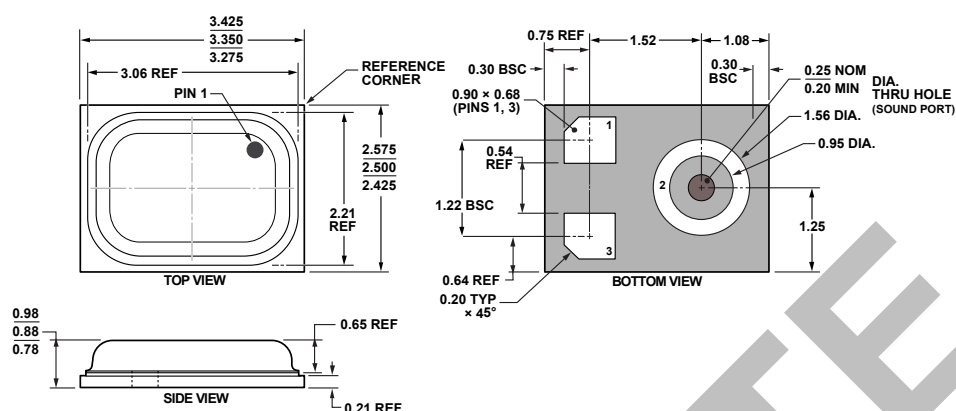
Figure 11. 3-Terminal Chip Array Small Outline No Lead Cavity [LGA_CAV] 3.35 mm x 2.50 mm Body (CE-3-2)
