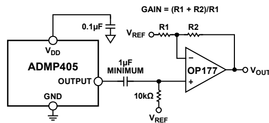
Figure 8. ADMP405 Connected to the OP177 Op Amp
