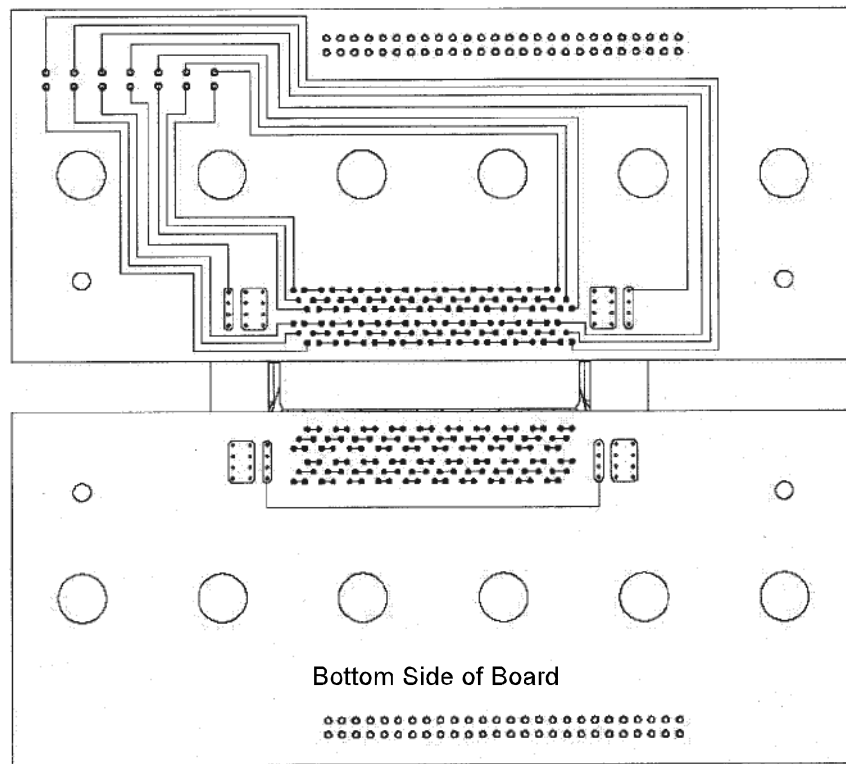
Figure 3 Low Level Contact Resistance Measurement Points
