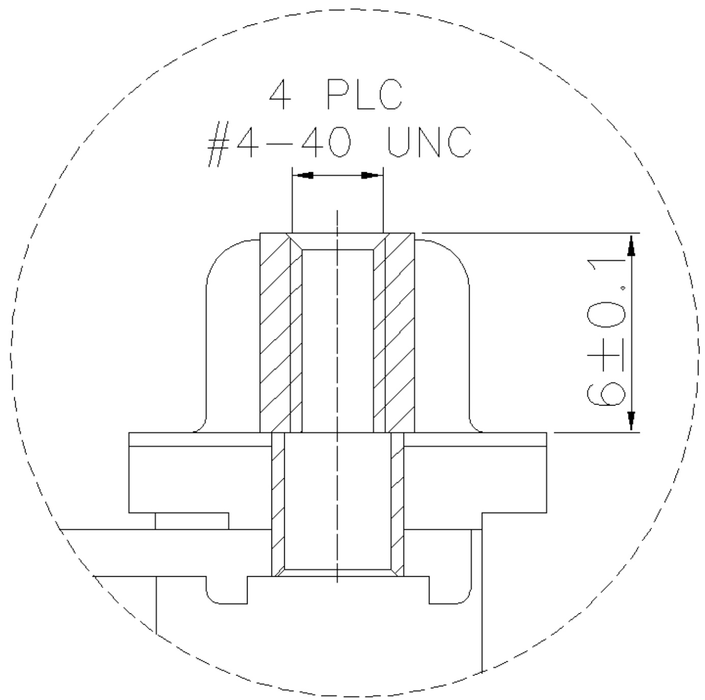
DETAIL A
