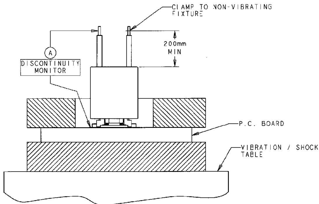
Figure 4 Vibration & Mechanical Shock Mounting Fixture
