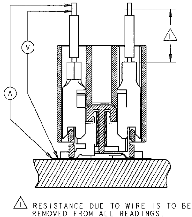
Figure 3 Dry Circuit Resistance Measurement Points
