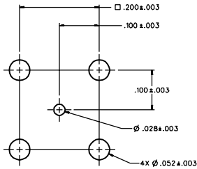
MOUNTING HOLE LAYOUT
