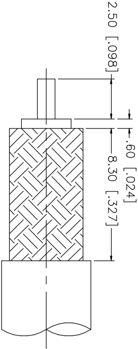
RECOMMENDED CABLE STRIPPING DIMENSIONS
