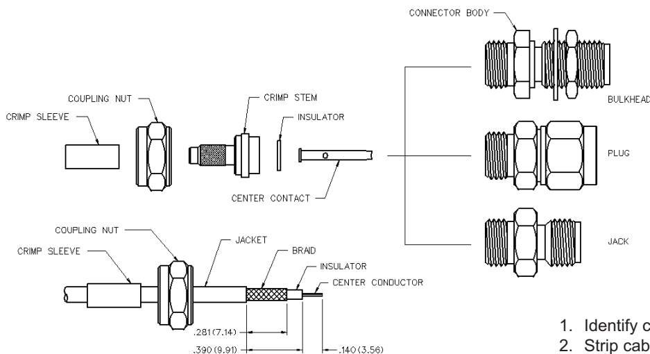
RG-178, RG-316 CABLE GROUP (142 SERIES)
