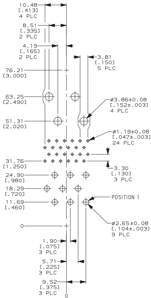
75A Middle Drawer Socket Side
