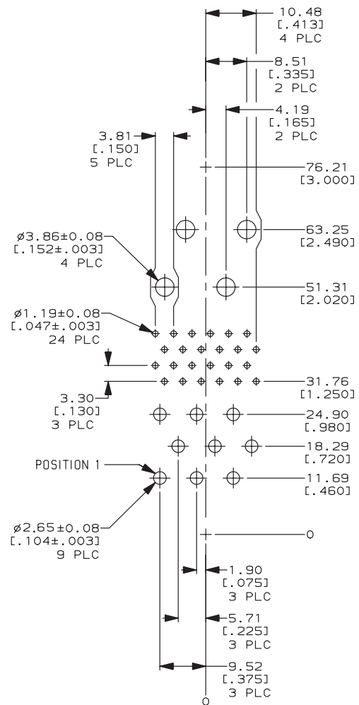
75A Middle Drawer Pin Side
