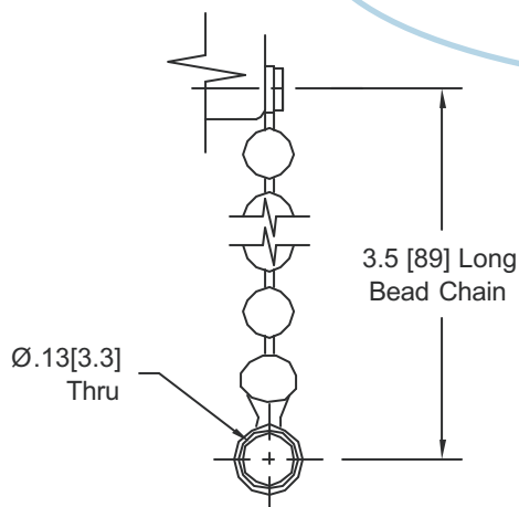
CHAIN DETAIL
