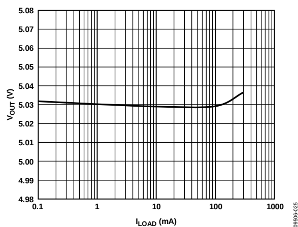
Figure 31. Output Voltage vs. Load Current, V_{OUT} = 5\text{ V} , Adjustable
