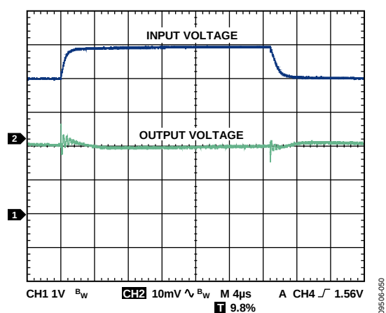
Figure 57. Line Transient Response, C_{IN} = 1\mu F , I_{LOAD} = 1mA , V_{OUT} = 1.8V
