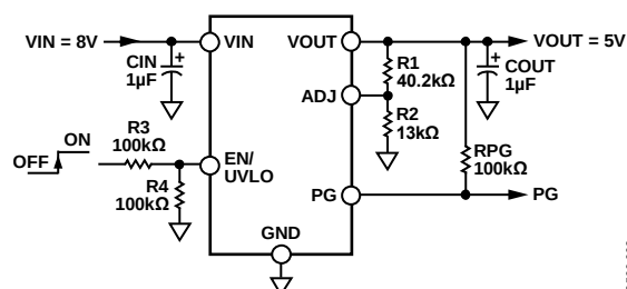
Figure 2. ADP7102 with Adjustable Output Voltage, 5 V
