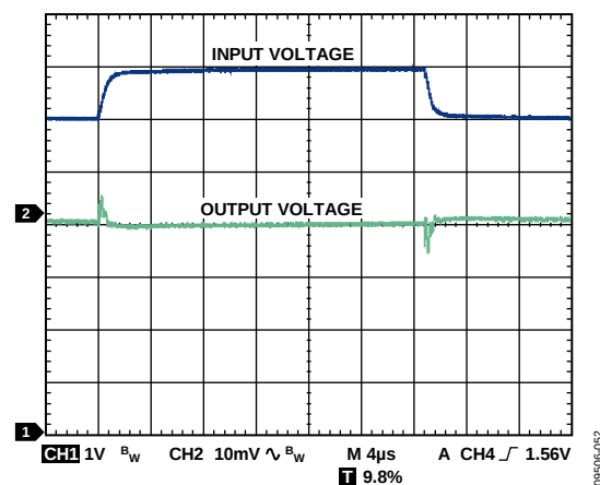
Figure 59. Line Transient Response, C_{IN} = 1\mu F , I_{LOAD} = 1mA , V_{OUT} = 5V
