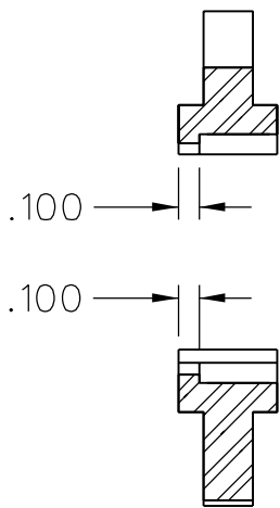
SECTION "C-C"
