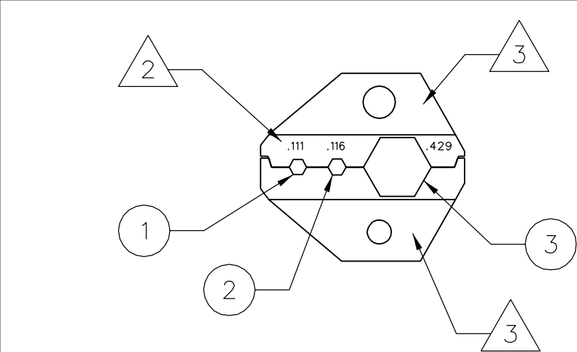
ASSEMBLED VIEW
