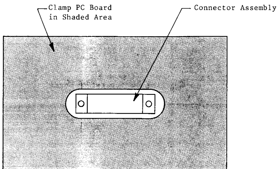
Figure 7 Mounting and Clamping Location for Vibration and Physical Shock
