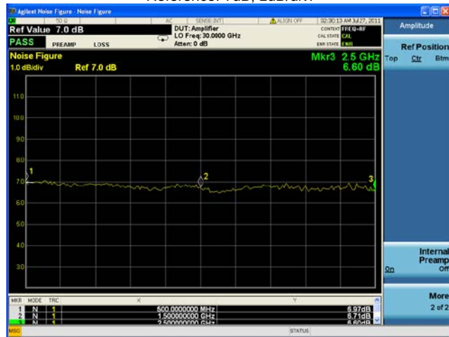
Plot 3 – Noise Figure
