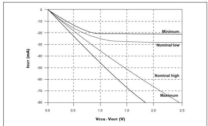
FIGURE D – REDUCED DRIVE PULL-UP CHARACTERISTICS
