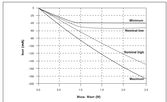
FIGURE B – FULL DRIVE PULL-UP CHARACTERISTICS
