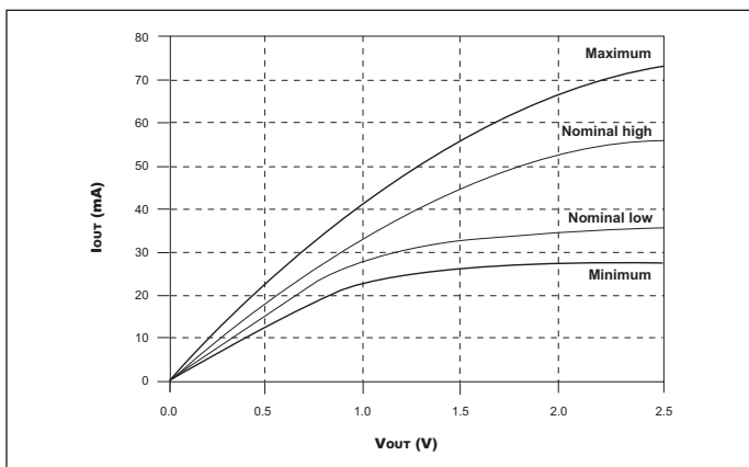
FIGURE C – REDUCED DRIVE PULL-DOWN CHARACTERISTICS
