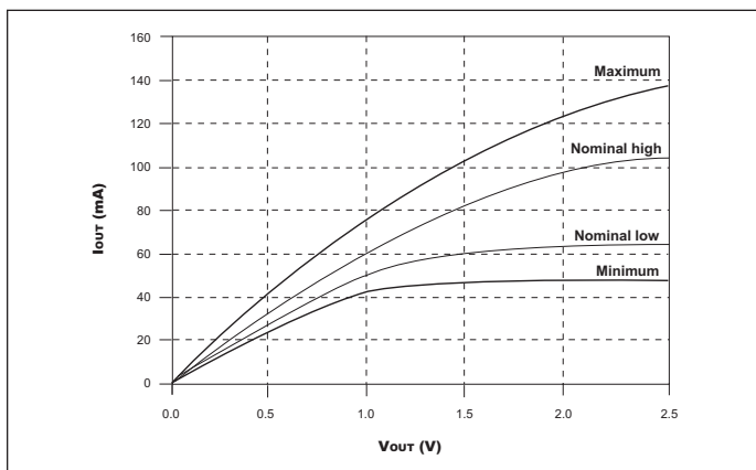
FIGURE A – FULL DRIVE PULL-DOWN CHARACTERISTICS
