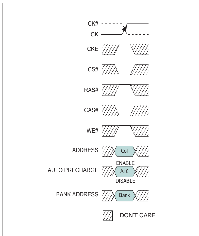
FIGURE 11 – READ COMMAND
