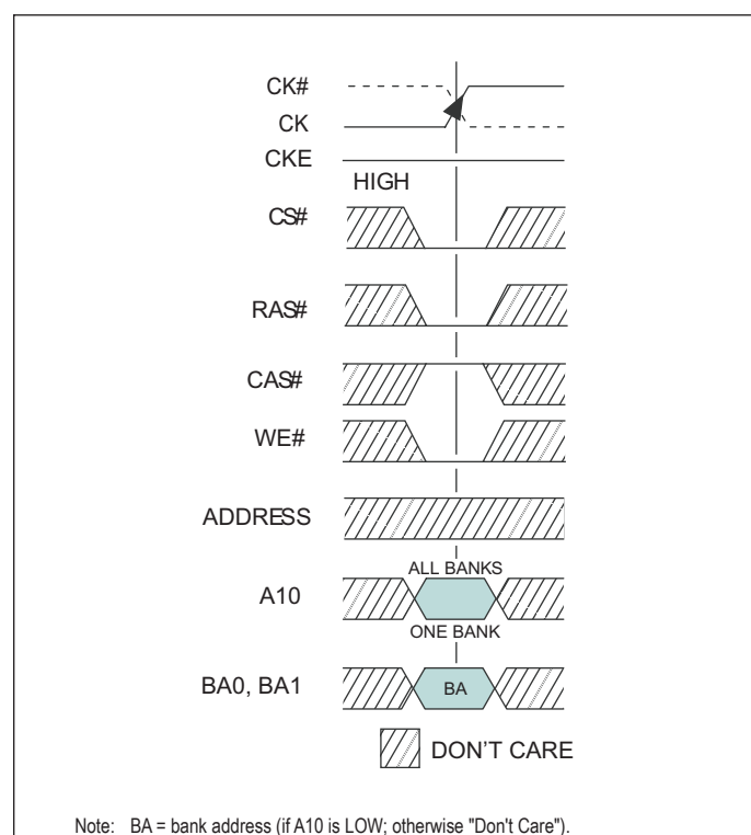
FIGURE 13 – PRECHARGE COMMAND
