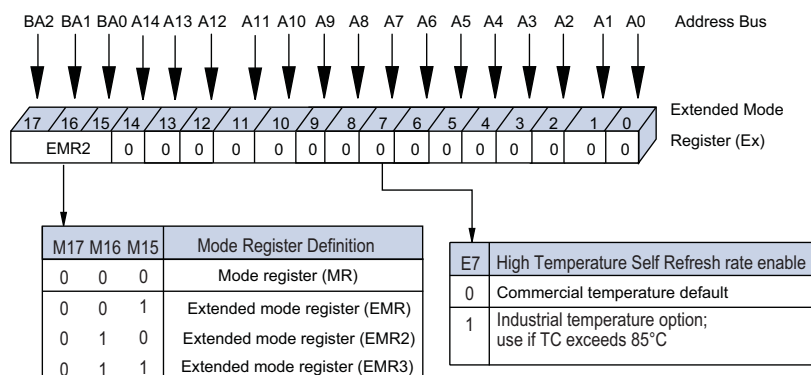
FIGURE 8 – EXTENDED MODE REGISTER 2 (EMR2) DEFINITION
