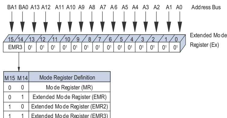
FIGURE 9 – EXTENDED MODE REGISTER 3 (EMR3) DEFINITION
