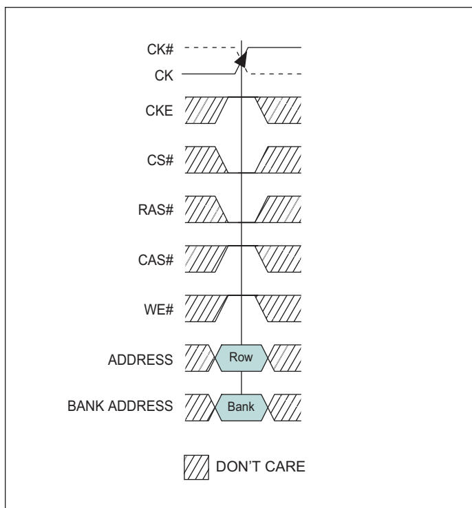
FIGURE 10 – ACTIVE COMMAND
