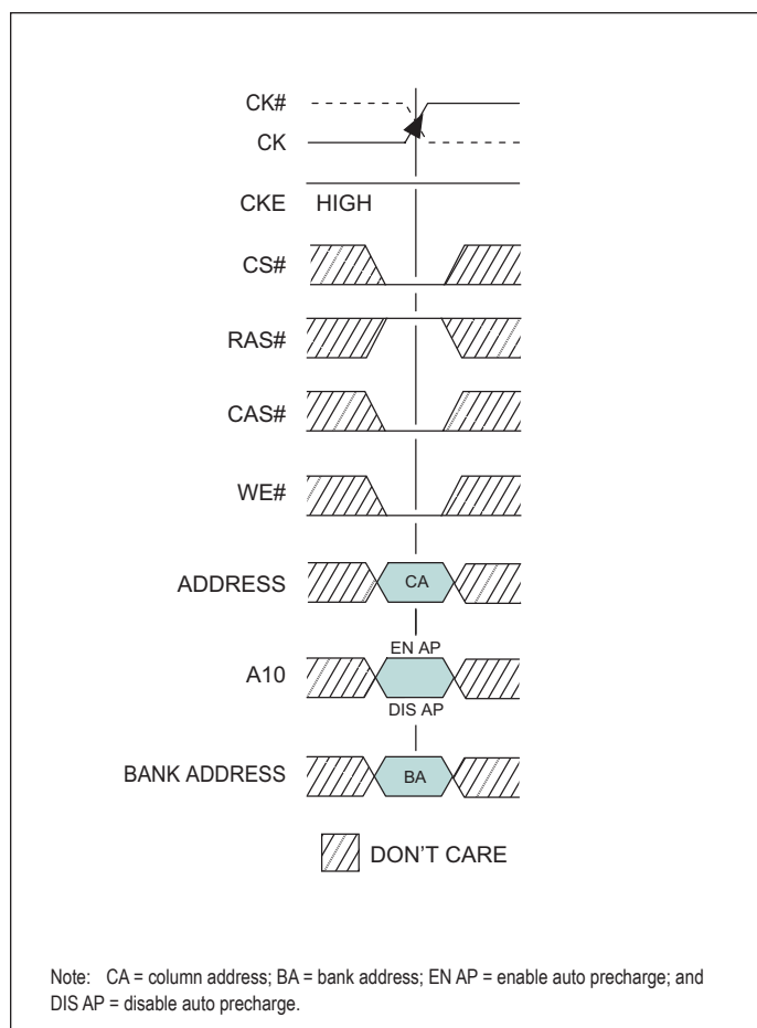
FIGURE 12 – WRITE COMMAND
