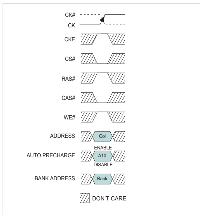
FIGURE 11 – READ COMMAND
