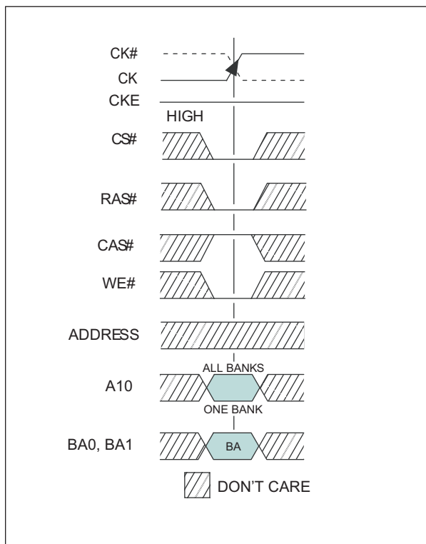
FIGURE 13 – PRECHARGE COMMAND
