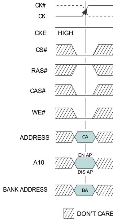
FIGURE 12 – WRITE COMMAND
