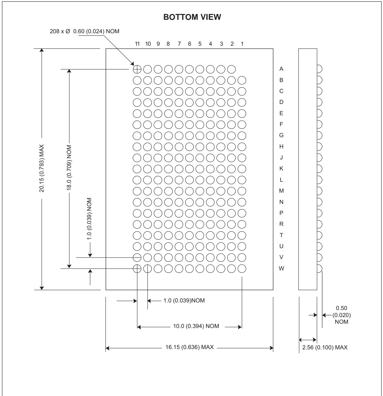
FIGURE 14 – PACKAGE DIMENSION: 208 PLASTIC BALL GRID ARRAY (PBGA)
