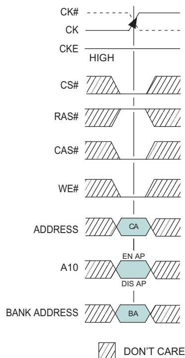
FIGURE 12 – WRITE COMMAND
