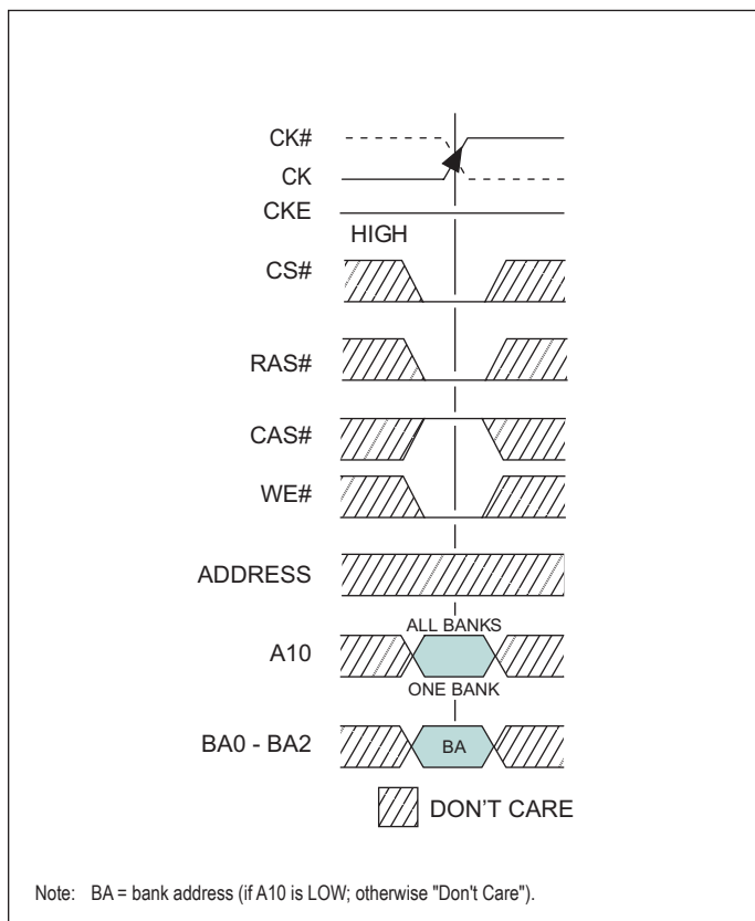
FIGURE 13 – PRECHARGE COMMAND
