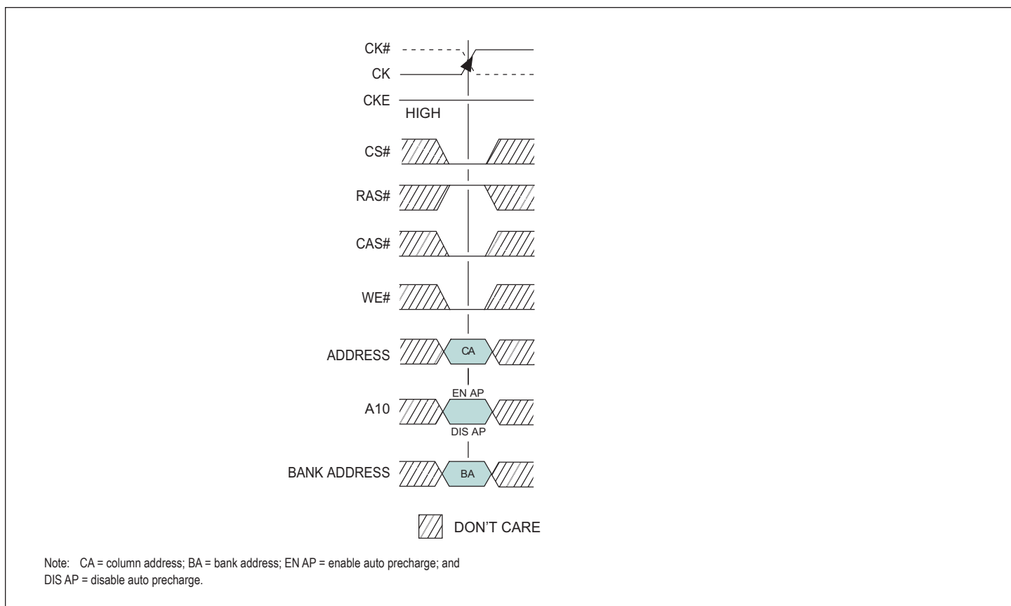
FIGURE 12 – WRITE COMMAND
