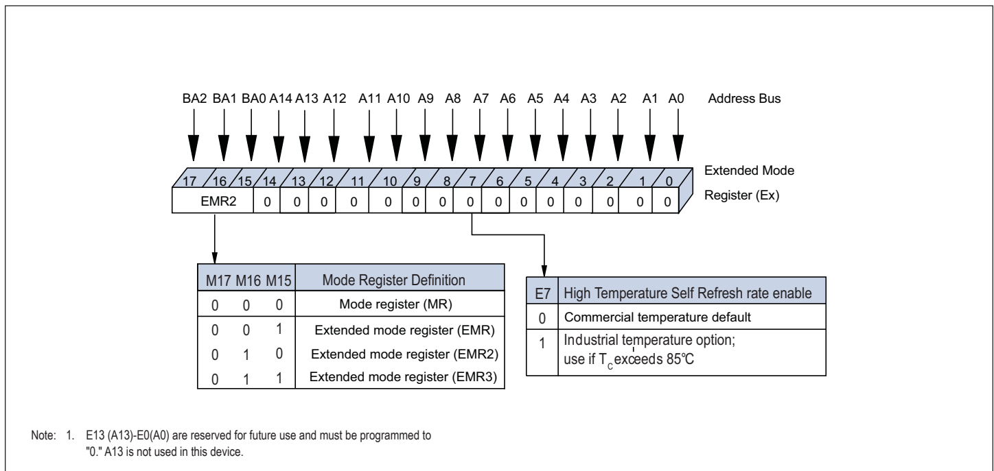
FIGURE 8 – EXTENDED MODE REGISTER 2 (EMR2) DEFINITION
