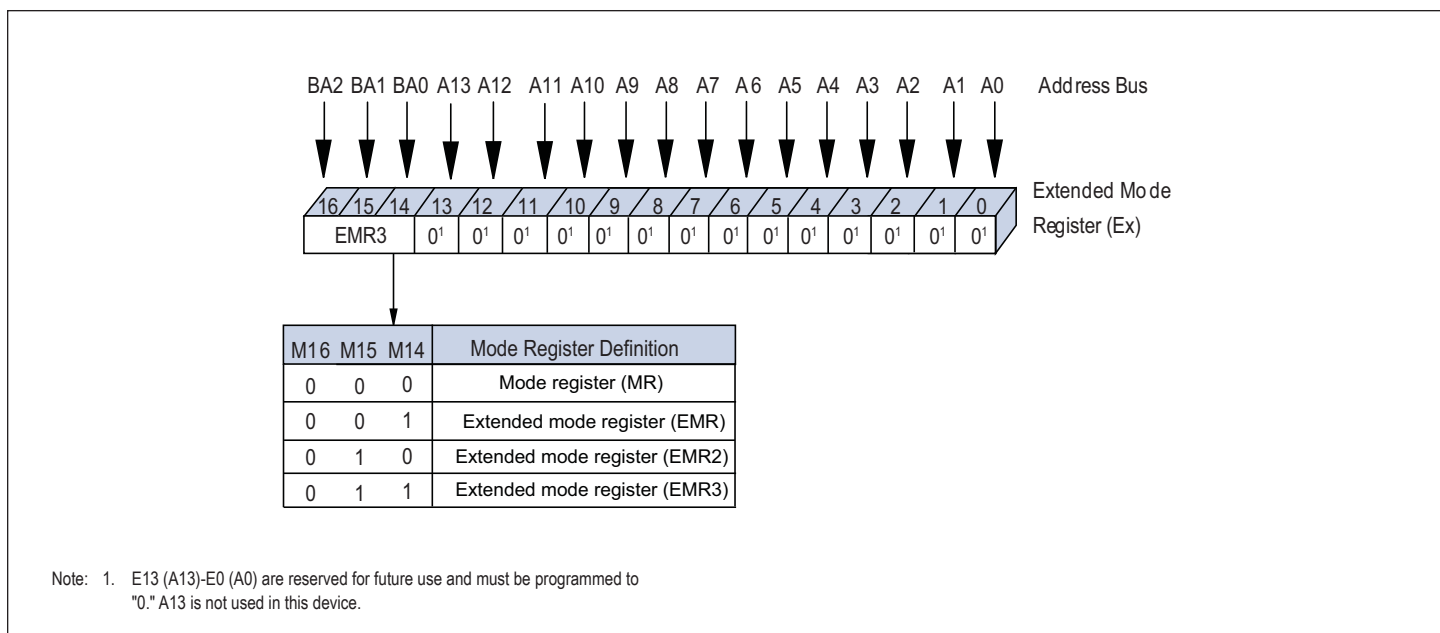
FIGURE 9 – EXTENDED MODE REGISTER 3 (EMR3) DEFINITION
