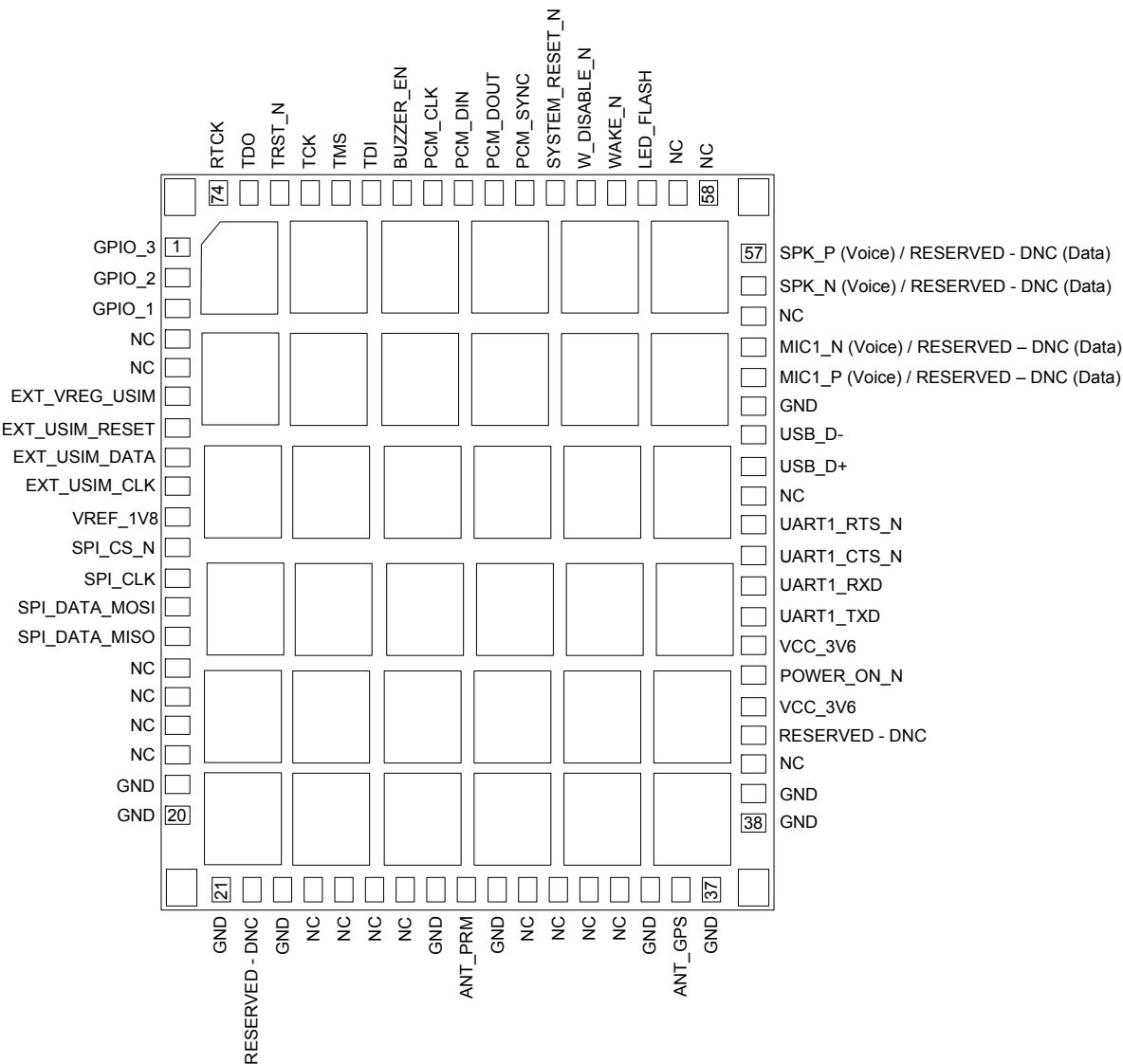
Figure 4-4: SL808X device pinouts 1
