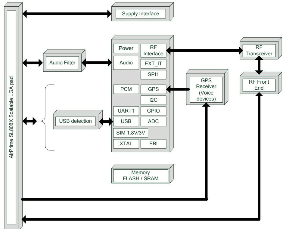
Figure 2-1: Functional architecture
