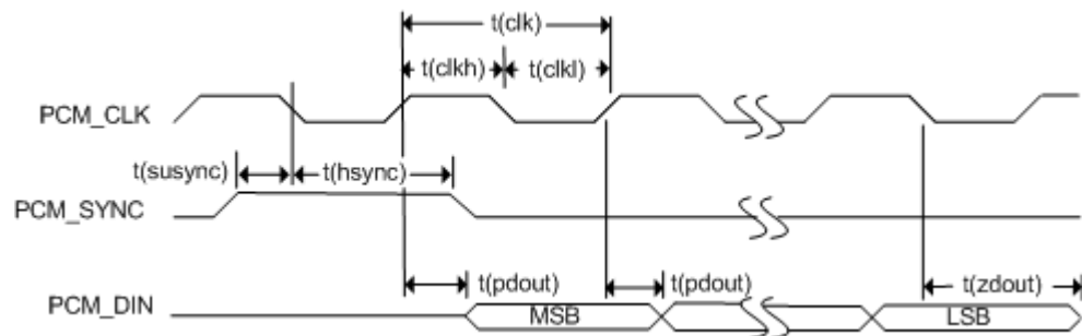
Figure 4-15: Timing diagram—SL808x to external PCM_CODEC
