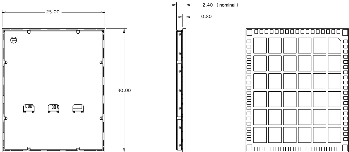
Figure 3-2: Dimensioned view
