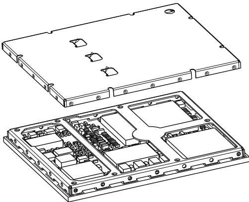
Figure 3-1: Exploded view
