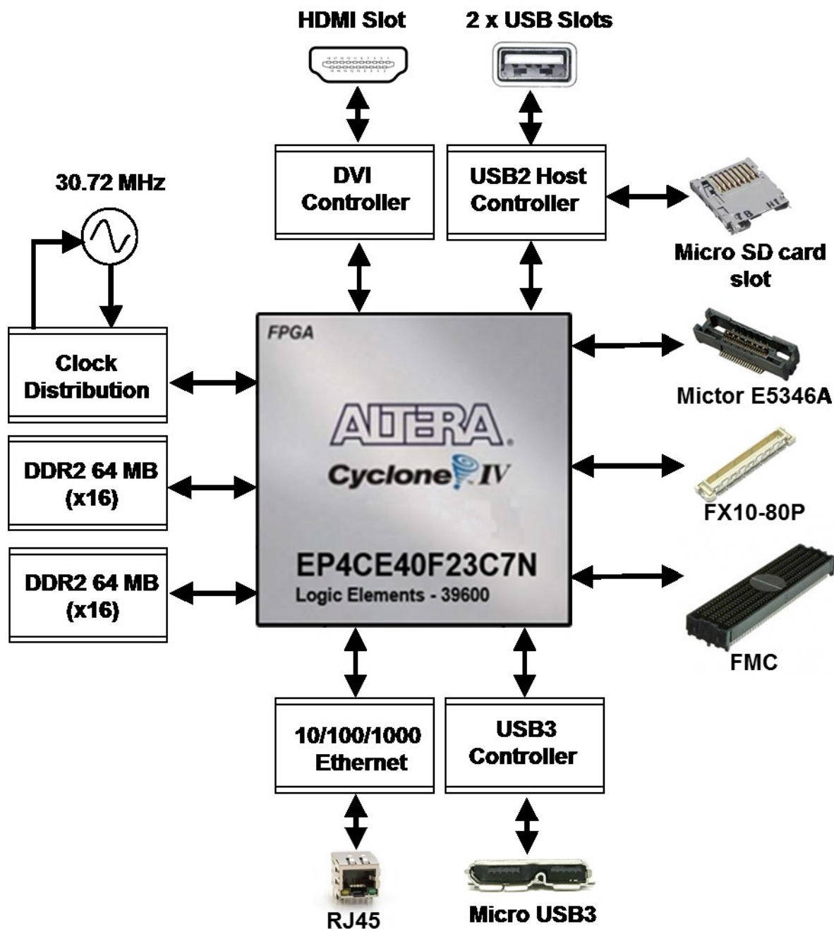
Figure 3 STREAM Development Board Block Diagram
