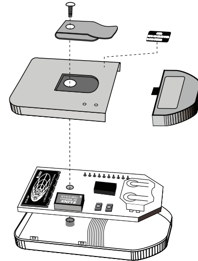
Figure 8: OTX-***-HH-CP8-HS Assembly
