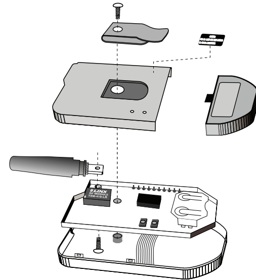
Figure 8: OTX-***-HH-LR8-HS Assembly
