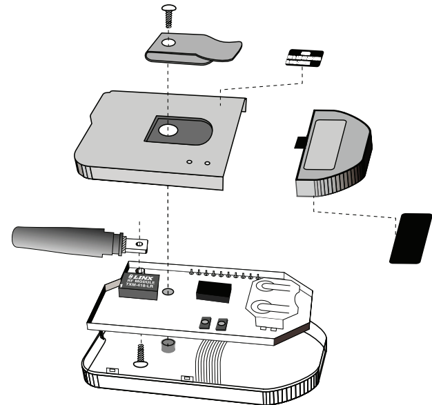
Figure 8: OTX-***-HH-LR8-MS Assembly
