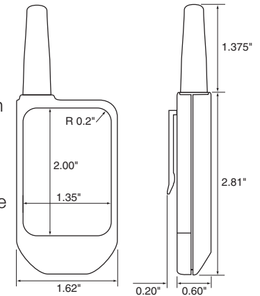
Figure 1: Package Dimensions
