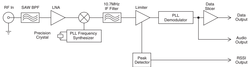
Figure 11: ES Series Receiver Block Diagram
