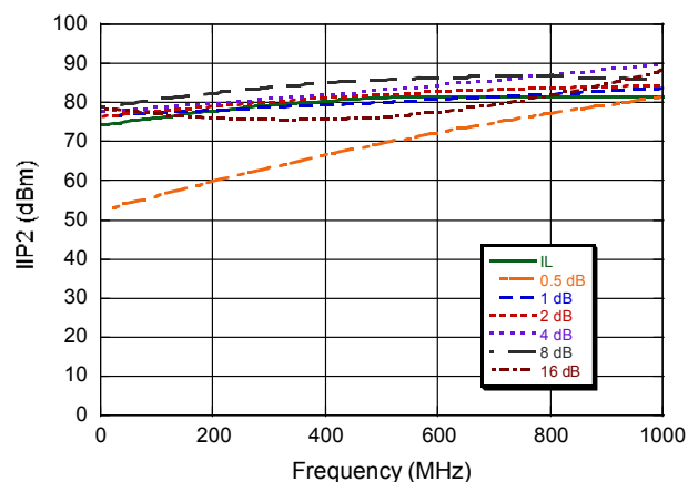
IIP2 vs. Frequency @ +85°C
