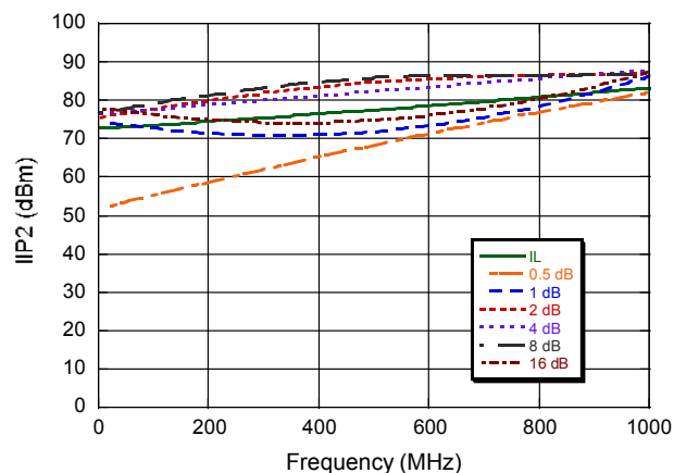
IIP2 vs. Frequency @ -40°C
