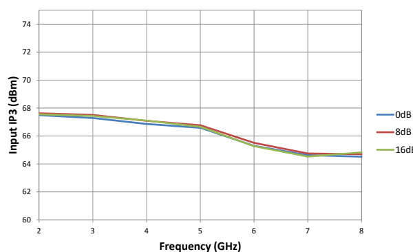
Figure 28. IIP3 vs. Attenuation Setting
