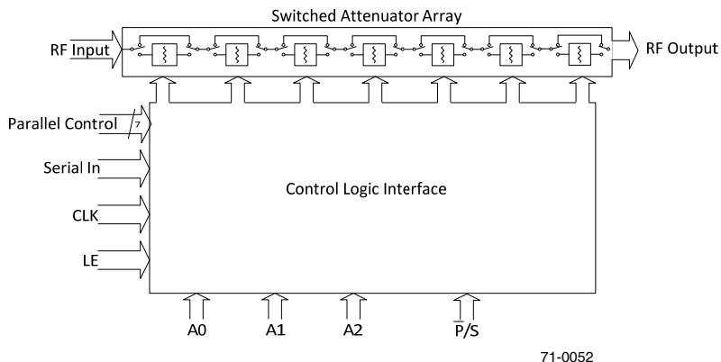
Figure 1. Functional Diagram
