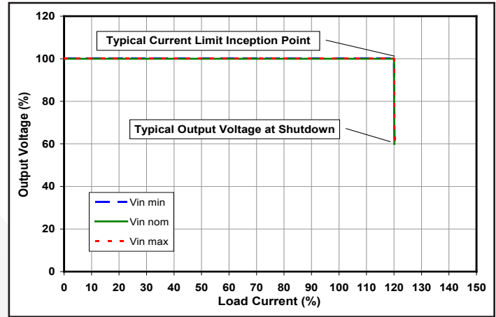
Common Figure 2: Output voltage vs. load current showing typical current limit inception curves and converter shutdown points.
