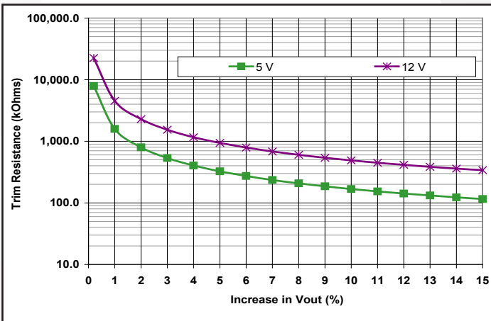
Common Figure 3: Trim graph for trim-up 5 and 12 V outputs.
