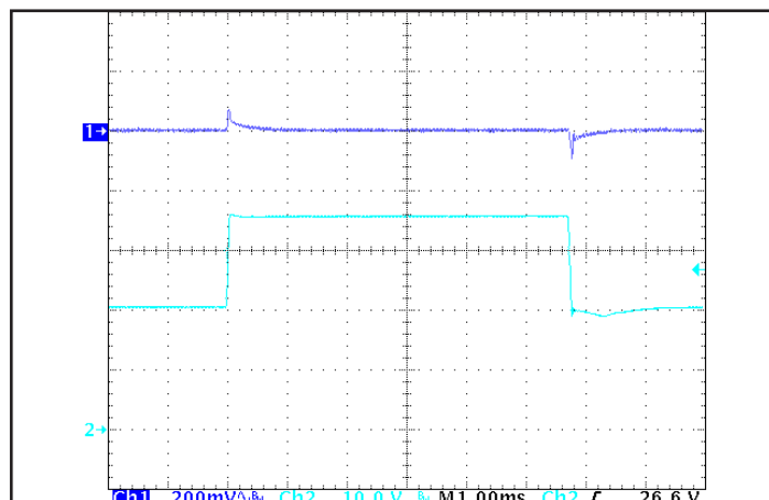
Figure 6: Output voltage response to step-change in input voltage (1000 V/ms). Load cap: 100 μF, electrolytic output capacitance. Ch 1: V out (200 mV/div), Ch 2: V in (10 V/div).
