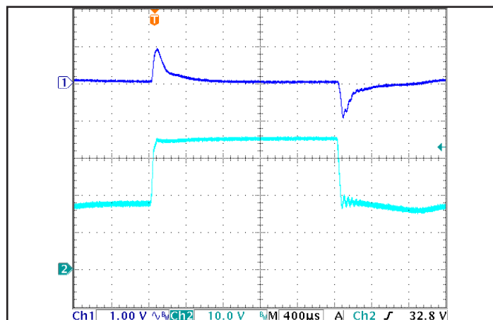
Figure 6: Output voltage response to step-change in input voltage (500 V/ms). Load cap: 100 μF, electrolytic output capacitance. Ch 1: V out (1 V/div), Ch 2: V in (10 V/div).
