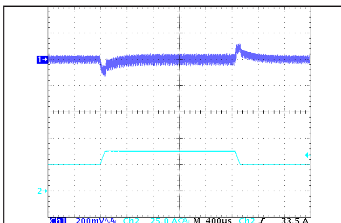
Figure 5: Output voltage response to step-change in load current (66%-100%-66% of Iout(max); dI/dt = 0.1 A/μs). Load cap: 1 μF ceramic capacitor. Ch 1: Vout (200 mV/div), Ch 2: Iout (25 A/div).
