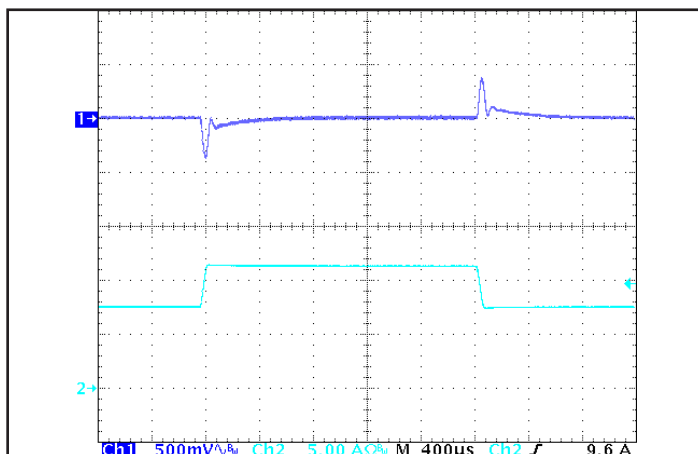
Figure 5: Output voltage response to step-change in load current (66%-100%-66% of Iout(max); dI/dt = 0.1 A/μs). Load cap: 1 μF ceramic capacitor. Ch 1: Vout (500 mV/div), Ch 2: Iout (5 A/div).
