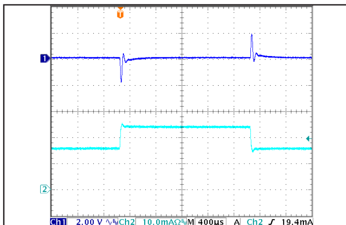
Figure 5: Output voltage response to step-change in load current (66%-100%-75% of I out (max); dI/dt = 0.1 A/μs). Load cap: 1 μF ceramic capacitor. Ch 1: V out (2 V/div), Ch 2: I out (10 mA/div).
