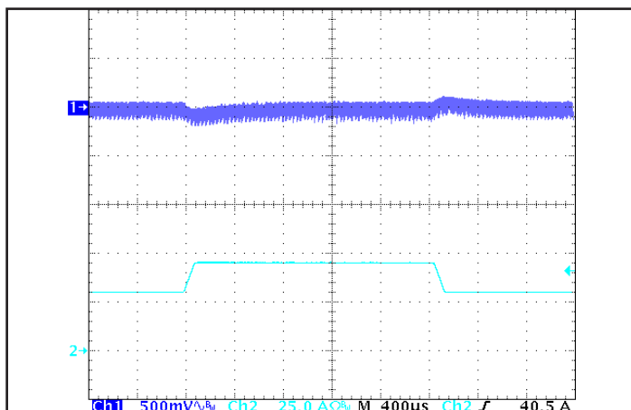
Figure 5: Output voltage response to step-change in load current (66%-100%-66% of I out (max); dI/dt = 0.1 A/μs). Load cap: 1 μF ceramic capacitor. Ch 1: V out (500 mV/div), Ch 2: I out (25 A/div).
