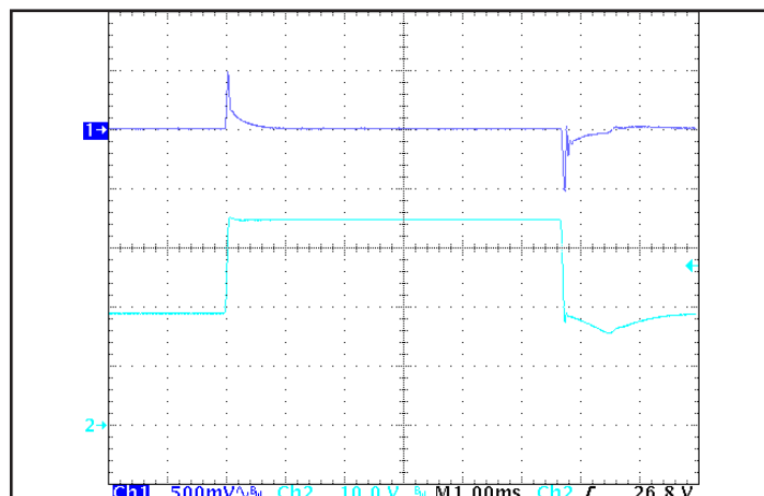
Figure 6: Output voltage response to step-change in input voltage (1000 V/ms). Load cap: 100 μF, electrolytic output capacitance. Ch 1: Vout (500 mV/div), Ch 2: Vin (10 V/div).
