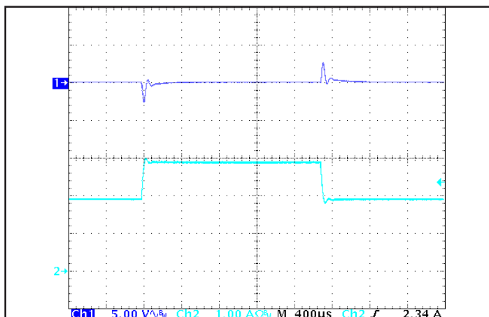
Figure 5: Output voltage response to step-change in load current (66%-100%-66% of I out (max); dI/dt = 0.1 A/μs). Load cap: 1 μF ceramic capacitor. Ch 1: V out (5 V/div), Ch 2: I out (1 A/div).
