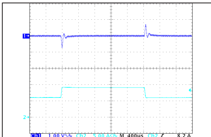
Figure 5: Output voltage response to step-change in load current (66%-100%-66% of Iout(max); dI/dt = 0.1 A/μs). Load cap: 1 μF ceramic capacitor. Ch 1: Vout (1 V/div), Ch 2: Iout (5 A/div).
