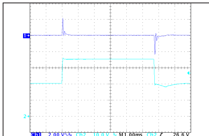
Figure 6: Output voltage response to step-change in input voltage (500 V/ms). Load cap: 100 μF, electrolytic output capacitance. Ch 1: V out (2 V/div), Ch 2: V in (10 V/div).
