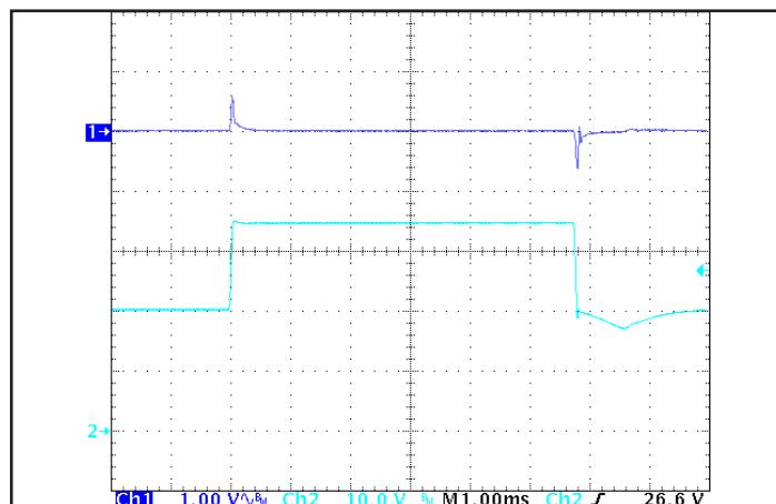
Figure 6: Output voltage response to step-change in input voltage (1000 V/ms). Load cap: 100 μF electrolytic output capacitance. Ch 1: Vout (1 V/div), Ch 2: Vin (10 V/div).
