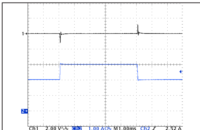
Figure 5: Output voltage response to step-change in load current (50%-75%-50% of Iout(max); dI/dt = 0.08 A/μs). Load cap: 1 μF ceramic capacitor. Ch 1: Vout (2 V/div), Ch 2: Iout (1 A/div).
