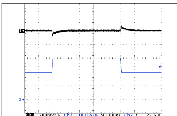
Figure 5: Output voltage response to step-change in load current (50%-75%-50% of I out (max); dI/dt = 0.2A/μs). Load cap: 15μF tantalum cap and 1μF ceramic cap. Ch 1: (200mV/div, Ch 2: I out (10A/div).
