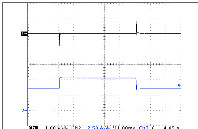
Figure 5: Output voltage response to step-change in load current (50%-75%-50% of Iout(max); dI/dt = 0.1 A/μs). Load cap: 1 μF ceramic and 15 μF tantalum capacitors. Ch 1: Vout (1 V/div), Ch 2: Iout (2.5 A/div).
