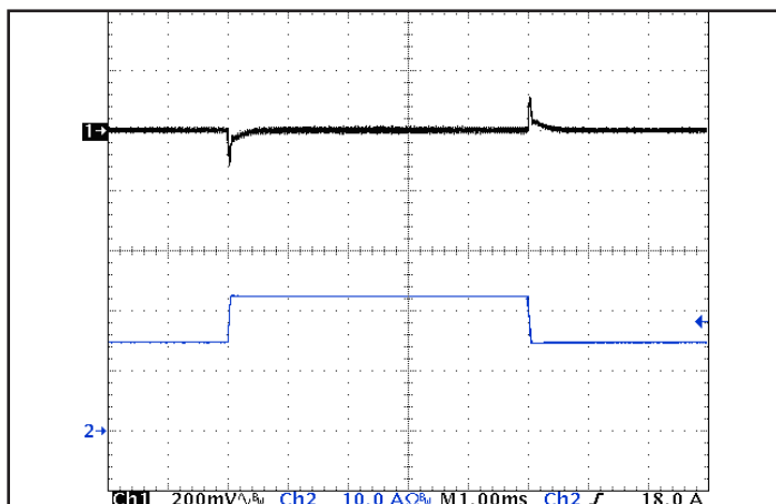
Figure 5: Output voltage response to step-change in load current (50%-75%-50% of Iout(max); dI/dt = 0.2A/μs). Load cap: 15μF tantalum cap and 1μF ceramic cap. Ch 1: Vout(200 mV/div), Ch 2: Iout (10 A/div).
