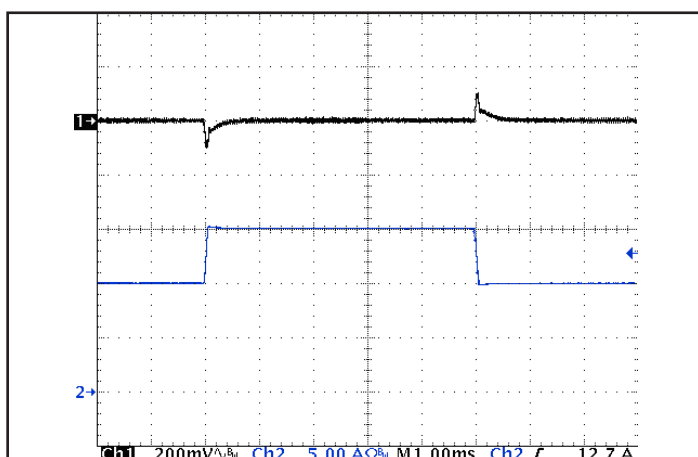
Figure 5: Output voltage response to step-change in load current (50%-75%-50% of Iout(max); dI/dt = 0.1A/μs. Load cap: 15μF tantalum cap and 1μF ceramic cap. Ch 1: Vout (200 mV/div), Ch 2: Iout (5 A/div).
