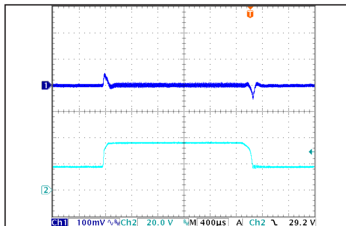
Figure 6: Output voltage response to step-change in input voltage (nominal to maximum, 250 V/ms). Load cap: 1μF ceramic capacitor. Ch 1: Vout, Ch 2: Vin.
