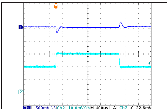
Figure 5: Output voltage response to step-change in load current (50%-75%-50% of I out (max); dI/dt = 0.2 A/μs). Load cap: 1μF ceramic capacitor. Ch 1: V out , Ch 2: I out (2 A/div).
