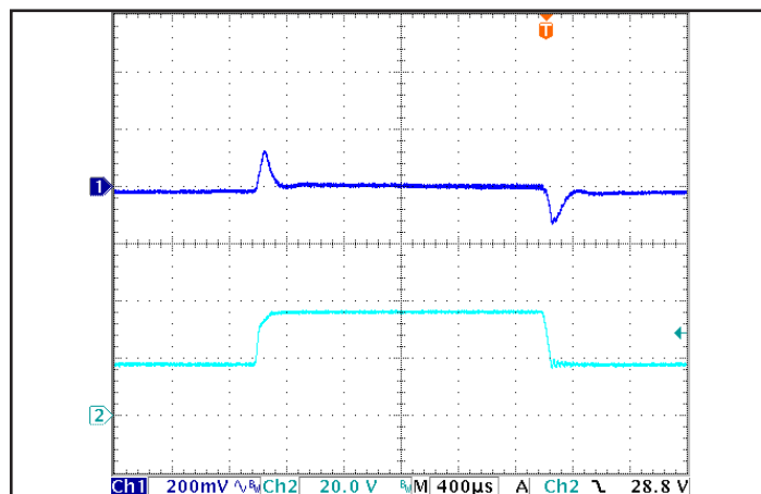
Figure 6: Output voltage response in the SM version to step-change in input voltage (25V/ms). Load cap: 100 µF electrolytic output capacitance. Ch 1: Vout (200 mV/div), Ch 2: Vin (20 V/div).
