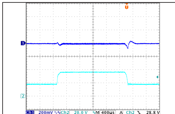
Figure 6: Output voltage response in the SM version to step-change in input voltage (250 V/ms). Load cap: 100 μF, electrolytic output capacitance. Ch 1: Vout (200 mV/div), Ch 2: Vin (20 V/div).
