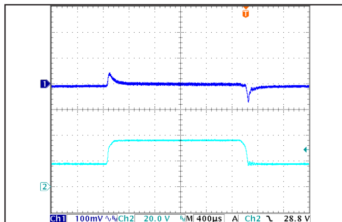
Figure 6: Output voltage response in the SM version to step-change in input voltage (25V/ms). Load cap: 100 µF, electrolytic output capacitance. Ch 1: Vout (100 mV/div), Ch 2: Vin (20 V/div).
