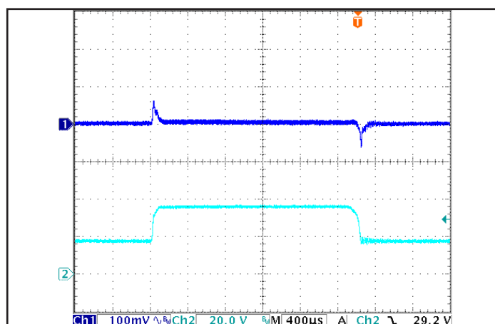
Figure 6: Output voltage response in the SM version to step-change in input voltage (25V/ms). Load cap: 100 µF, electrolytic output capacitance. Ch 1: Vout (100 mV/div), Ch 2: Vin (20 V/div).
