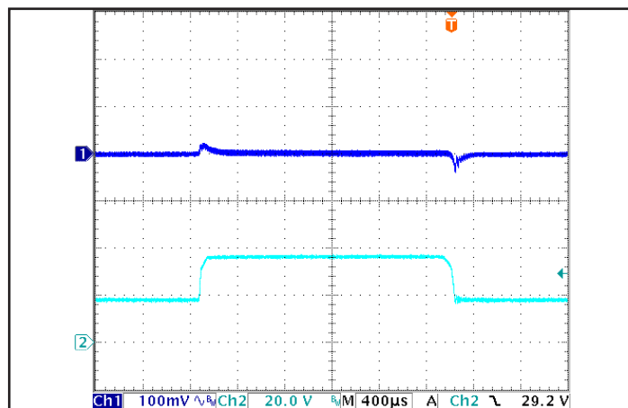
Figure 6: Output voltage response in the SM version to step-change in input voltage (25V/μs). Load cap: 100 μF, electrolytic output capacitance. Ch 1: Vout (100 mV/div), Ch 2: Vin (20 V/div).
