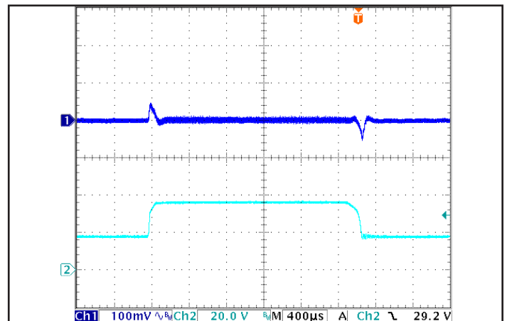
Figure 6: Output voltage response in the SM version to step-change in input voltage (25V/ms). Load cap: 100 μF, electrolytic output capacitance. Ch 1: V out (100 mV/div), Ch 2: V in (20 V/div).
