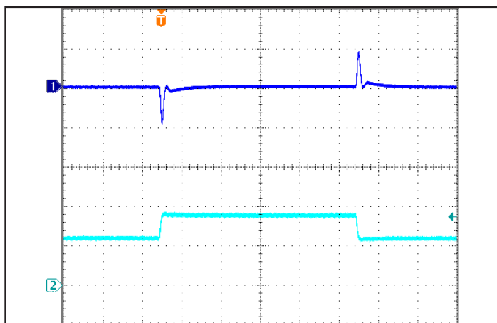
Figure 5: Output voltage response to step-change in load current (66%-100%-66% of Iout(max); dI/dt = 0.2 \text{ A}/\mu\text{s} ). Load cap: 1 \mu\text{F} ceramic and 15 \mu\text{F} tantalum capacitors. Ch 1: Vout (200 mV/div), Ch 2: Iout (10 A/div).
