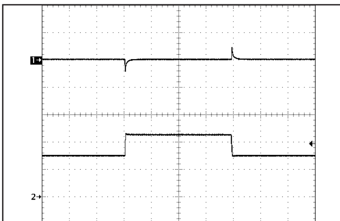
Figure 5: Output voltage response to step-change in load current (66%-100%-66% of Iout(max); dI/dt = 0.08 A/us). Load cap: 1 μF ceramic capacitor. Ch 1: Vout (2 V/div), Ch 2: Iout (2.5 A/div).
