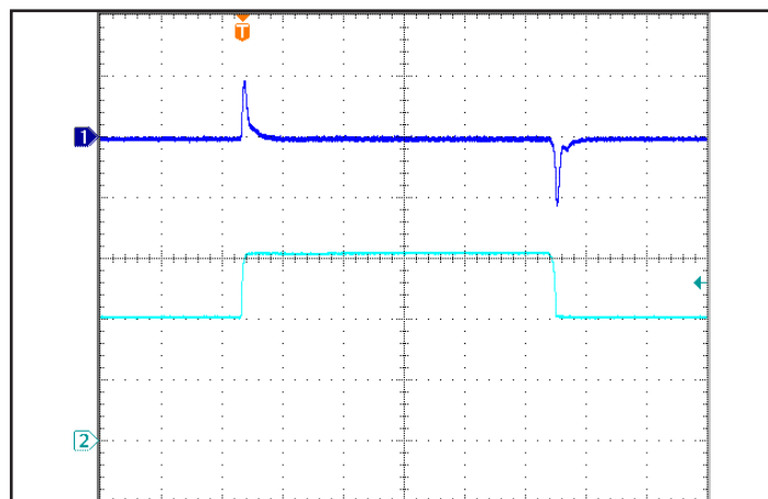
Figure 6: Output voltage response to step-change in input voltage (1000 V/ms). Load cap: 100 \mu\text{F} , electrolytic output capacitance. Ch 1: Vout (200 mV/div), Ch 2: Vin (50 V/div).
