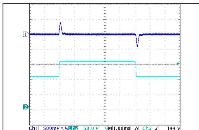
Figure 6: Output voltage response to step-change in input voltage (nominal to maximum input voltage), at Full Load current. Load cap: 1uF ceramic cap. Ch 1: V out , Ch 2: V in .
