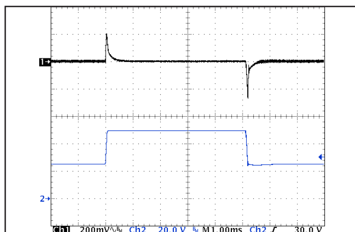
Figure 6: Output voltage response to step-change in input voltage (500 V/ms). Load cap: 100 μF, electrolytic output capacitance. Ch 1: V out (200 mV/div), Ch 2: V in (20 V/div).
