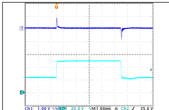
Figure 6: Output voltage response to step-change in input voltage (500 V/ms). Load cap: 100 μF, electrolytic output capacitance. Ch 1: Vout (1 V/div), Ch 2: Vin (20 V/div).
