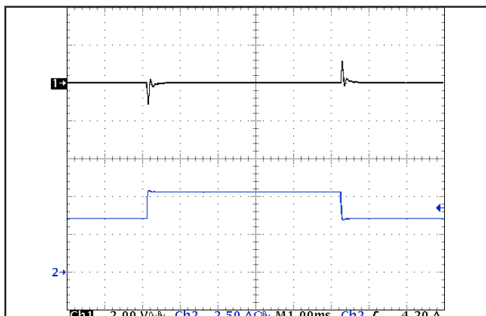
Figure 5: Output voltage response to step-change in load current (66%-100%-66% of I out(max) ; dI/dt = 0.1 A/μs). Load cap: 1 1/4F ceramic capacitor. Ch 1: V out (2 V/div), Ch 2: I out (2.5 A/div).
