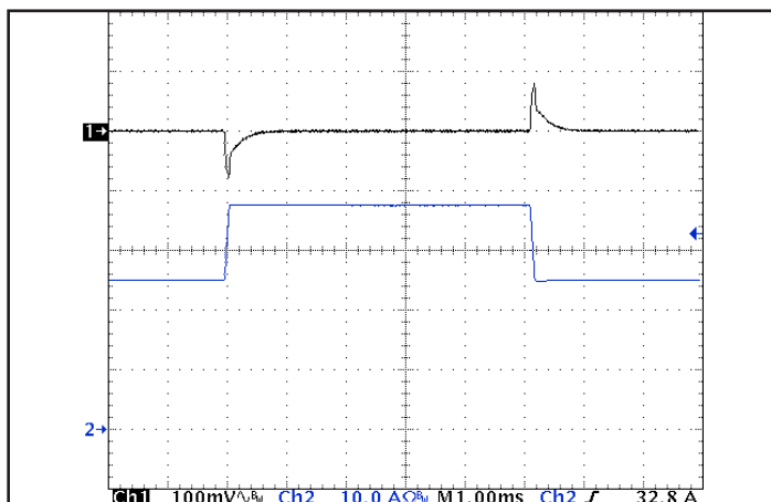
Figure 5: Output voltage response to step-change in load current (66%-100%-66% of I out (max); dI/dt = 0.2 A/μs). Load cap: 1 μF ceramic and 15 μF tantalum capacitors. Ch 1: V out (100 mV/div), Ch 2: I out (10 A/div).
