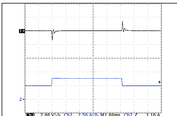
Figure 5: Output voltage response to step-change in load current (66%-100%-66% of I_{out(max)} ; dI/dt = 0.05 A/\mu s ). Load cap: 1 \mu F ceramic capacitor. Ch 1: V_{out} (2 V/div), Ch 2: I_{out} (2.5 A/div).
