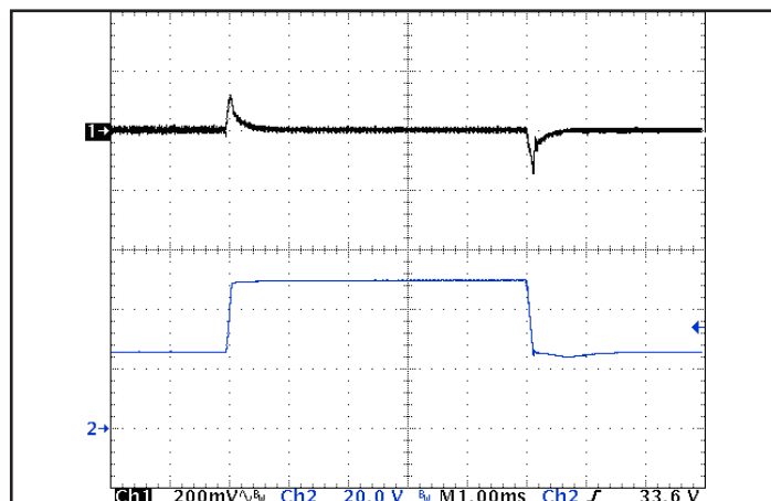
Figure 6: Output voltage response to step-change in input voltage (500 V/ms). Load cap: 100 μF, electrolytic output capacitance. Ch 1: V out (200 mV/div), Ch 2: V in (20 V/div).
