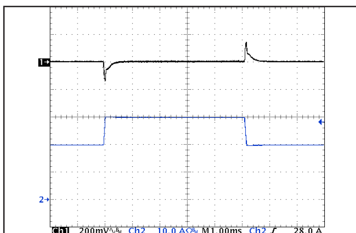
Figure 5: Output voltage response to step-change in load current (66%-100%-66% of I out (max); dI/dt = 0.1 A/μs). Load cap: 1 μF ceramic and 15 μF tantalum capacitors. Ch 1: V out (200 mV/div), Ch 2: I out (10 A/div).
