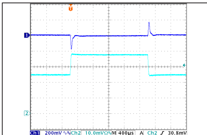
Figure 5: Output voltage response to step-change in load current (50%-75%-50% of I out (max); dI/dt = 0.1 A/μs). Load cap: 100 μF electrolytic cap and 1 μF ceramic cap. Ch 1: V out (200 mV/div), Ch 2: I out (2 A/div).
