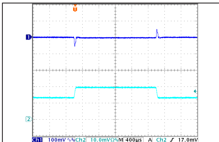
Figure 5: Output voltage response to step-change in load current (50%-75%-50% of Iout(max); dI/dt = 0.1 A/μs). Load cap: 100 μF electrolytic cap and 1 μF ceramic cap. Ch 1: Vout (100 mV/div), Ch 2: Iout (10 A/div).
