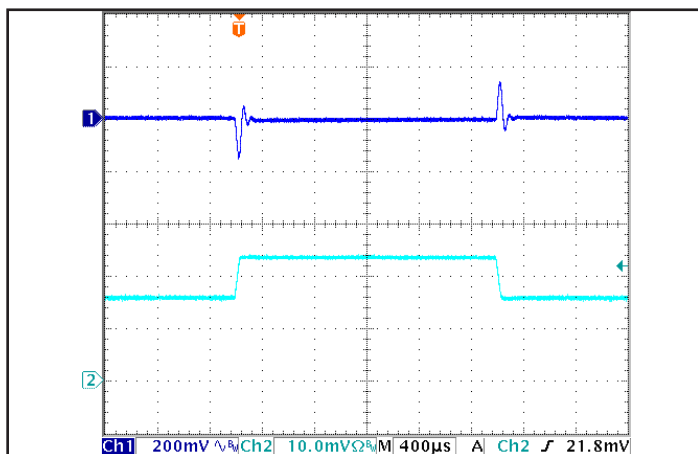
Figure 5: Output voltage response to step-change in load current (50%-75%-50% of Iout(max); dI/dt = 0.1 A/μs). Load cap: 100 μF electrolytic cap and 1 μF ceramic cap. Ch 1: Vout (200 mV/div), Ch 2: Iout (5 A/div).
