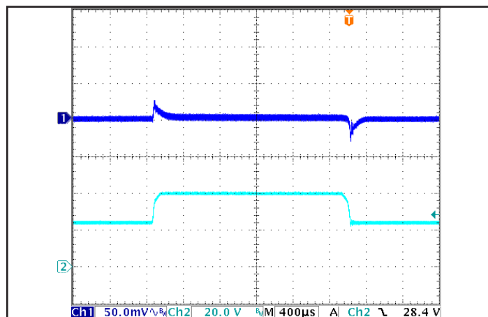
Figure 6: Output voltage response to step-change in input voltage (250 V/ms). Load cap: 100 μF, electrolytic output capacitance. Ch 1: Vout (50 mV/div), Ch 2: Vin (20 V/div).
