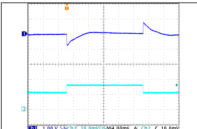
Figure 5: Output Voltage Response to Step-Change in Load Current (50%-75%-50% of I out (max); dI/dt = 0.1A/μs. Load cap: 100μF electrolytic cap and 1μF ceramic cap. Ch 1: V out , Ch 2: I out (5 A/div).
