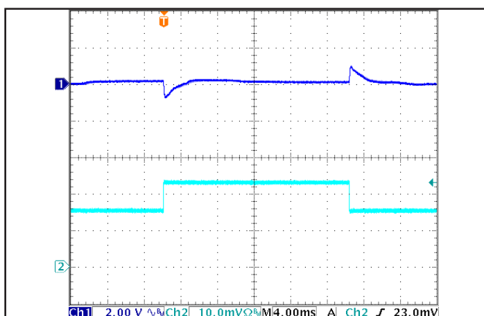
Figure 5: Output Voltage Response to Step-Change in Load Current (50%-75%-50% of Iout(max); dI/dt = 0.1A/μs). Load cap: 100μF electrolytic cap and 1μF ceramic cap. Ch 1: Vout, Ch 2: Iout (2 A/div).
