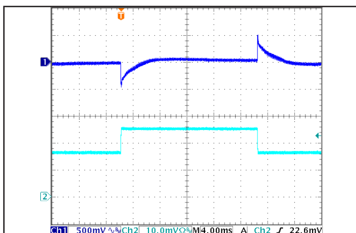
Figure 5: Output Voltage Response to Step-Change in Load Current (50%-75%-50% of Iout(max); dI/dt = 0.1A/μs. Load cap: 15μF tantalum cap and 1μF ceramic cap. Ch 1: Vout, Ch 2: Iout (5 A/div).
