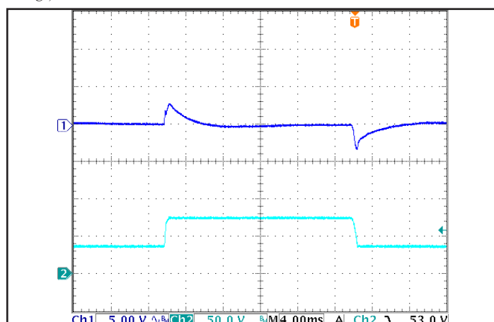
Figure 6: Output Voltage Response to Step-Change in Input Voltage (250 V/ms), at Max. load current. Load cap: 330μF electrolytic cap and 1μF ceramic cap. Ch 1: Vout, Ch 2: Vin.
