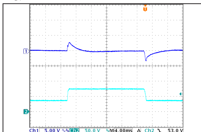
Figure 6: Output Voltage Response to Step-Change in Input Voltage (250 V/ms), at Max. load current. Load cap: 330μF electrolytic cap and 1μF ceramic cap. Ch 1: Vout, Ch 2: Vin.
