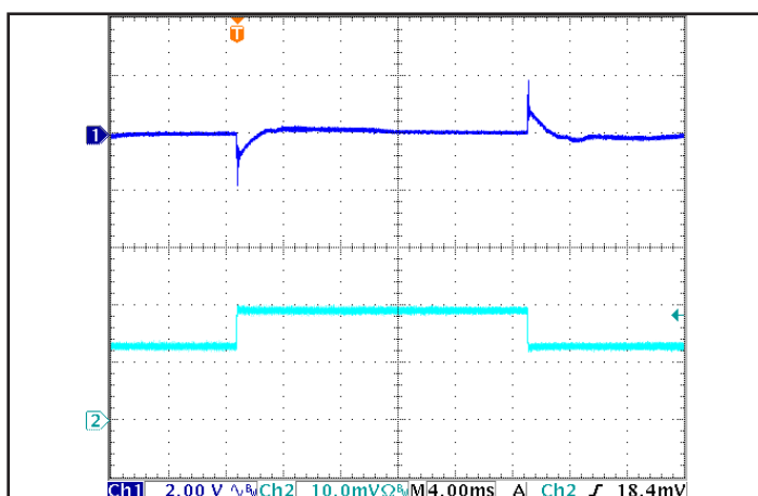
Figure 5: Output Voltage Response to Step-Change in Load Current (50%-75%-50% of Iout(max); dI/dt = 0.1A/μs. Load cap: 100μF electrolytic cap and 1μF ceramic cap. Ch 1: Vout, Ch 2: Iout (2.0 A/div).
