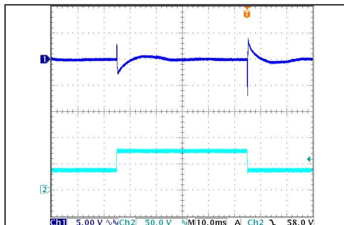
Figure 6: Output Voltage Response to Step-Change in Input Voltage (250 V/ms), at Max. load current. Load cap: 330μF tantalum cap and 1μF ceramic cap. Ch 1: Vout, Ch 2: Vin.
