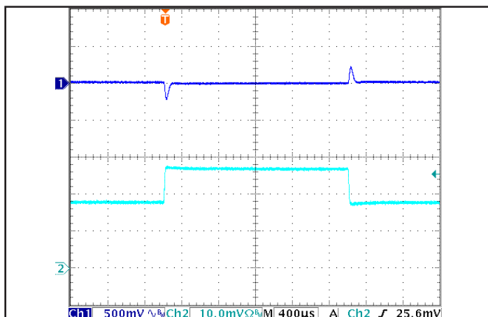
Figure 5: Output voltage response to step-change in load current for Mega version (50%-75%-50% of I out (max); dI/dt = 0.1 A/μs). Load cap: 100 μF electrolytic capacitor. Ch 1: V out (500 mV/div), Ch 2: I out (2 A/div)
