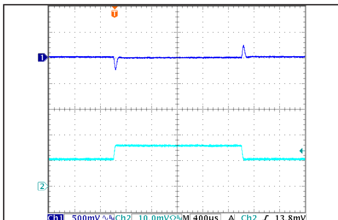
Figure 5: Output voltage response to step-change in load current for Mega version (50%-75%-50% of Iout(max); dI/dt = 0.1 A/μs). Load cap: 100 μF electrolytic capacitor. Ch 1: Vout (500 mV/div), Ch 2: Iout (5 A/div)
