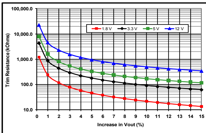
Common Figure 3: Trim-Up Graph for 5.0 to 15V outputs.
