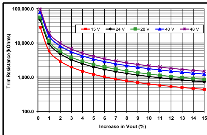
Common Figure 3: Trim-Up Graph for 24 to 50V outputs.
