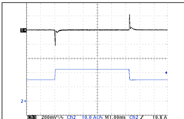
Figure 5: Output voltage response to step-change in load current (66%-100%-66% of Iout(max); dI/dt = 0.1 A/μs). Load cap: 15μF tantalum and 1uF ceramic capacitors. Ch 1: Vout, Ch 2: Iout (10 A/div).
