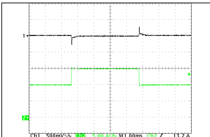
Figure 5: Output voltage response to step-change in load current (66%-100%-66% of Iout(max); dI/dt = 0.1A/us). Load cap: 15μF tantalum cap and 1μF ceramic cap. Ch 1: Vout, Ch 2: Iout.
