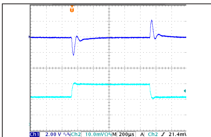
Figure 5: Output voltage response to step-change in load current (65%-100%-65% of I out (max); dI/dt = 0.2 A/μs). Load cap: 1μF ceramic capacitor. Ch 1: V out , Ch 2: I out .
