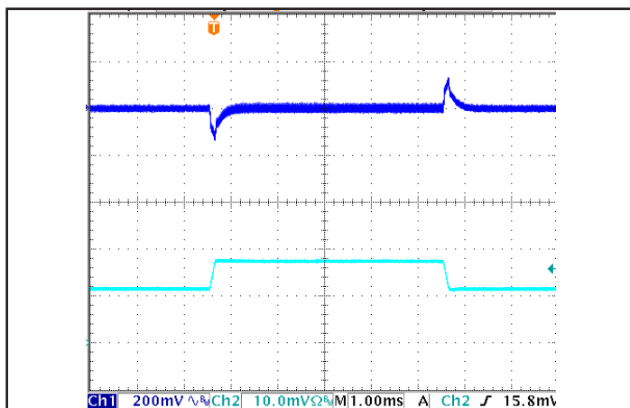
Figure 5: Output voltage response to step-change in load current (70%-100%-70% of Iout(max); dI/dt = 0.2 A/μs). Load cap: 15μF tantalum and 1uF ceramic capacitors. Ch 1: Vout, Ch 2: Iout.
