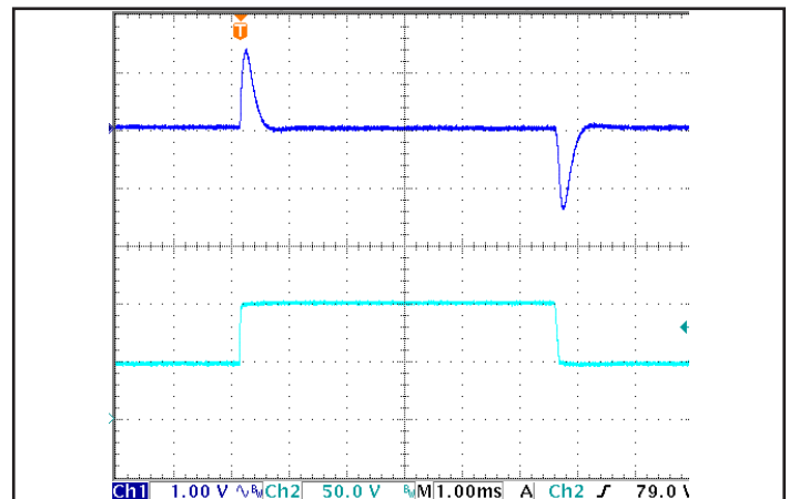
Figure 6: Output voltage response to step-change in input voltage (nominal to maximum, 250 V/ms). Load cap: 1 \mu F ceramic capacitor. Ch 1: V_{out} , Ch 2: V_{in} .
