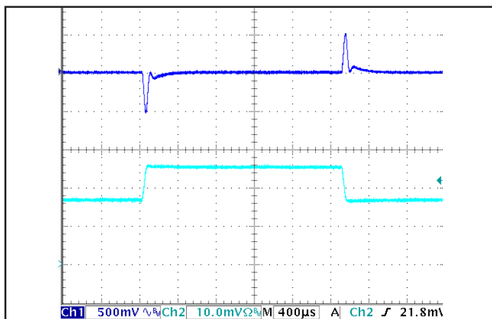
Figure 5: Output voltage response to step-change in load current (65%-100%-65% of I out (max); dI/dt = 0.2 A/μs). Load cap: 15μF tantalum and 1uF ceramic capacitors. Ch 1: V out , Ch 2: I out (5A/div).
