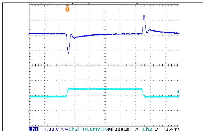
Figure 5: Output voltage response to step-change in load current (65%-100%-65% of Iout(max); dI/dt = 0.2 A/μs). Load cap: 1μF ceramic capacitor. Ch 1: Vout, Ch 2: Iout (2A/div).
