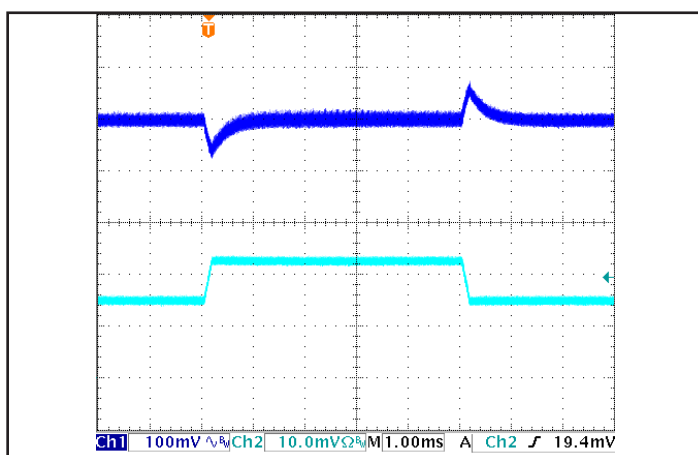
Figure 5: Output voltage response to step-change in load current (60%-90%-60% of I out (max); dI/dt = 0.2 A/μs). Load cap: 15μF tantalum and 1uF ceramic capacitors. Ch 1: V out , Ch 2: I out .
