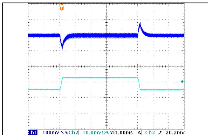
Figure 5: Output voltage response to step-change in load current (65%-100%-65% of Iout(max); dI/dt = 0.2 A/μs). Load cap: 15μF tantalum and 1uF ceramic capacitors. Ch 1: Vout, Ch 2: Iout.
