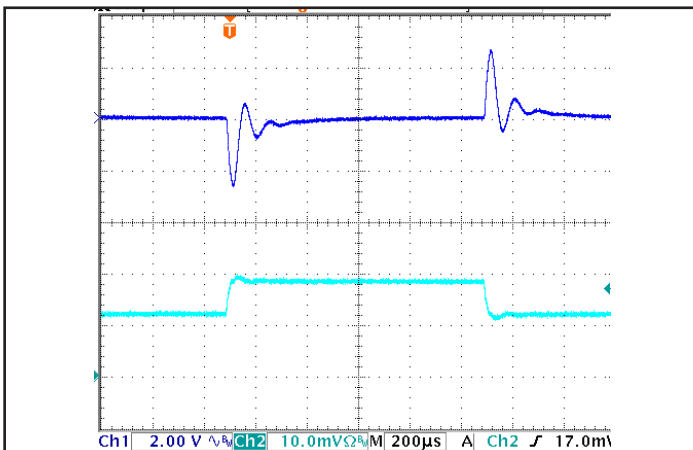
Figure 5: Output voltage response to step-change in load current (65%-100%-65% of I_{out(max)} ; dI/dt = 0.2 A/\mu s ). Load cap: 1 \mu F ceramic capacitor. Ch 1: V_{out} , Ch 2: I_{out} .
