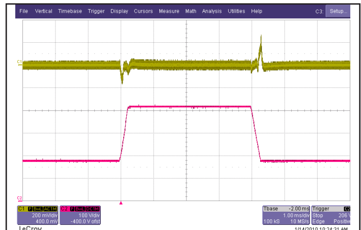
Figure 6: Output voltage response to step-change in input voltage (180V - 425V - 180V), at 50A load current. Load cap: 15μF tantalum capacitor and 1μF ceramic cap. Ch 1: Vout (200mV/div), Ch 2: Vin (100V/div).
