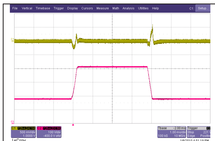
Figure 6: Output voltage response to step-change in input voltage (180V - 425V - 180V), at 20A load current. Load cap: 15μF tantalum capacitor and 1μF ceramic cap. Ch 1: V out (500mV/div), Ch 2: V in (100V/div).
