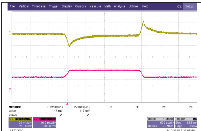
Figure 5: Output voltage response to step-change in load current (50%-75%-50% of Iout(max); dI/dt = 0.1A/μs). Load cap: 15μF tantalum cap and 1μF ceramic cap. Ch 1: Vout (100mV/div), Ch 2: Iout (20A/div).
