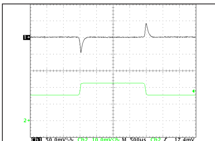
Figure 5: Output voltage response to step-change in load current (50%-75%-50% of Iout(max); dI/dt = 0.1A/μs). Load cap: 15μF, 100 mΩ ESR tantalum cap and 1μF ceramic cap. Ch 1: Vout (50mV/div), Ch 2: Iout (10A/div).
