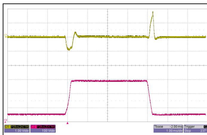
Figure 6: Output voltage response to step-change in input voltage (180 V - 425 V - 180 V) with 250 μs rise/fall time. Load cap: 15μF, 100 mΩ ESR tantalum cap and 1μF ceramic cap. Ch 1: Vout (1V/div). Ch 2: Vin (100V/div).
