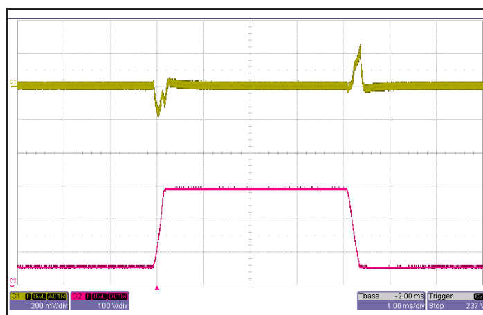
Figure 6: Output voltage response to step-change in input voltage (180 V - 425 V - 180 V) with 250 μs rise/fall time. Load cap: 15μF, 100 mΩ ESR tantalum cap and 1μF ceramic cap. Ch 1: V out (200mV/div). Ch 2: V in (100V/div).
