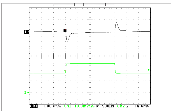
Figure 5: Output voltage response to step-change in load current (50%-75%-50% of Iout(max); dI/dt = 0.1A/μs). Load cap: 15μF, 100 mΩ ESR tantalum cap and 1μF ceramic cap. Ch 1: Vout (1V/div), Ch 2: Iout (1A/div).
