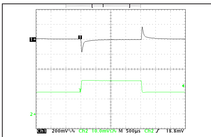
Figure 5: Output voltage response to step-change in load current (50%-75%-50% of I out (max); dI/dt = 0.1A/μs). Load cap: 15μF, 100 mΩ ESR tantalum cap and 1μF ceramic cap. Ch 1: V out (200mV/div), Ch 2: I out (10A/div).
