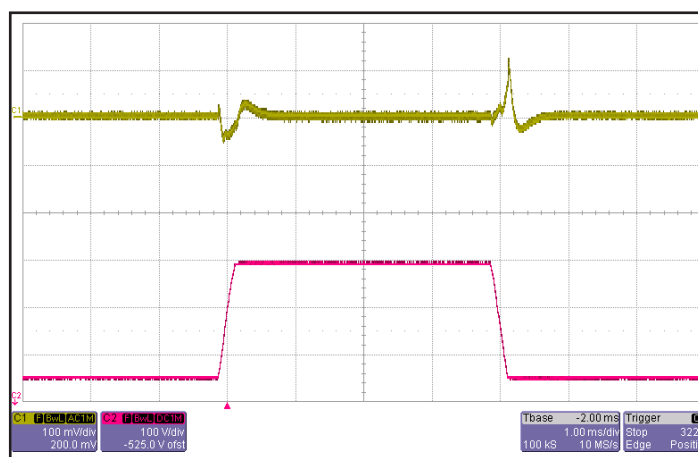
Figure 6: Output voltage response to step-change in input voltage (180 V - 425 V - 180 V) with 250 μs rise/fall time. Load cap: 15μF, 100 mΩ ESR tantalum cap and 1μF ceramic cap. Ch 1: Vout (100mV/div). Ch 2: Vin (100V/div).
