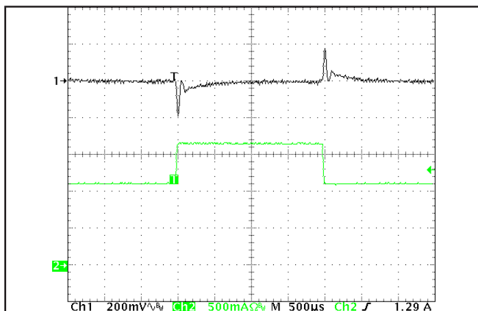
Figure 5: Output voltage response to step-change in load current (50%-75%-50% of Iout(max); dI/dt = 0.03A/μs. Load cap: 15μF tantalum cap and 1μF ceramic cap. Ch 1: Vout, Ch 2: Iout.
