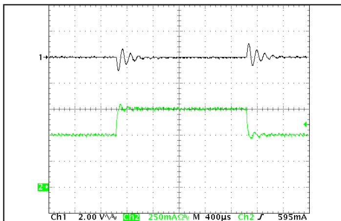
Figure 5: Output voltage response to step-change in load current (50%-75%-50% of Iout(max); dI/dt = 0.05A/μs). Load cap: 1μF ceramic cap. Ch 1: Vout, Ch 2: Iout.
