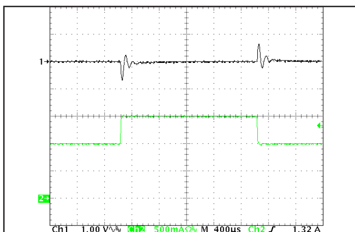
Figure 5: Output voltage response to step-change in load current (50%-75%-50% of Iout(max); dI/dt = 0.05A/μs). Load cap: 1μF ceramic cap. Ch 1: Vout, Ch 2: Iout.
