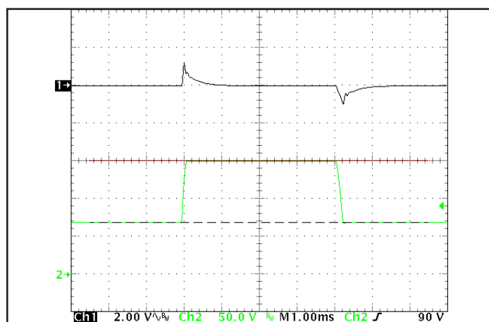
Figure 6: Output voltage response to step-change in input voltage (1000 V/ms), at Max. load current. Load cap: 1μF ceramic cap. Ch 1: Vout, Ch 2: Vin.
