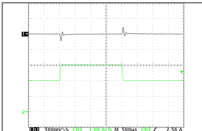
Figure 5: Output voltage response to step-change in load current (50%-75%-50% of I out (max); dI/dt = 0.05A/μs). Load cap: 15μF tantalum cap and 1μF ceramic cap. Ch 1: V out , Ch 2: I out .
