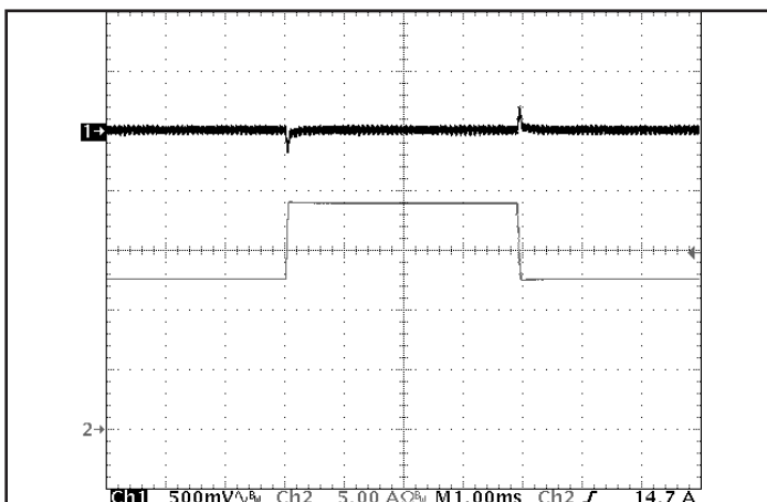
Figure 5: Output voltage response to step-change in load current (66%-100%-66% of I out (max); dI/dt = 0.1 A/μs). Load cap: 1 μF ceramic and 15 μF tantalum capacitors. Ch 1: V out (500 mV/div), Ch 2: I out (5 A/div).
