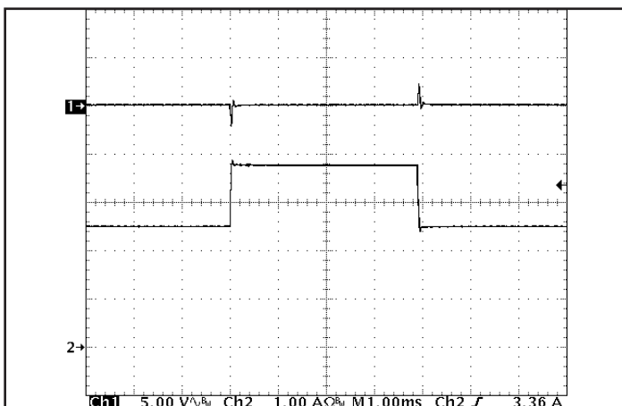
Figure 5: Output voltage response to step-change in load current (66%-100%-66% of I out (max); dI/dt = 0.05 A/μs). Load cap: 1 μF ceramic capacitor. Ch 1: V out (5 V/div), Ch 2: I out (1 A/div).
