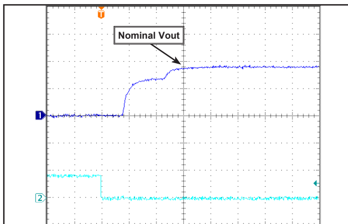
Common Figure 1: Typical startup waveform. Input voltage pre-applied, ON/OFF Pin on Ch 2. Timescale: 5ms/div.
