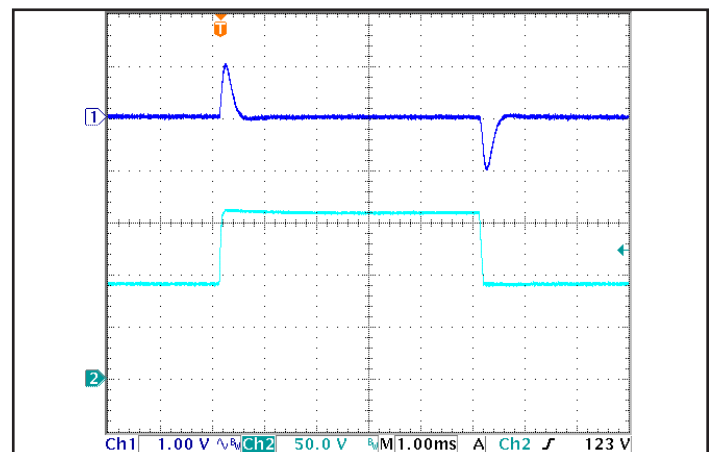
Figure 6: Output voltage response to step-change in input voltage (1000 V/ms). Load cap: 100 μF electrolytic output capacitance. Ch 1: V in (1 V/div), Ch 2: V out (50 V/div).
