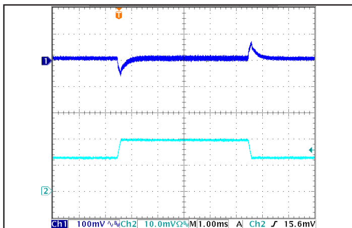
Figure 5: Output voltage response to step-change in load current (50%-75%-50% of I out (max); dI/dt = 0.1 A/μs). Load cap: 1 μF ceramic and 15 μF tantalum capacitors. Ch 1: V out (100 mV/div), Ch 2: I out (20 A/div).
