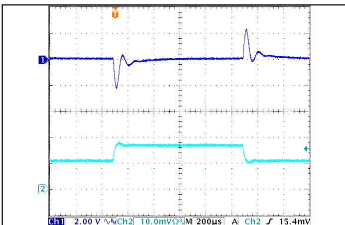
Figure 5: Output voltage response to step-change in load current (50%-75%-50% of I out (max); dI/dt = 0.05 A/μs). Load cap: 1 μF ceramic capacitor. Ch 1: V out (2 V/div), Ch 2: I out (2 A/div).
