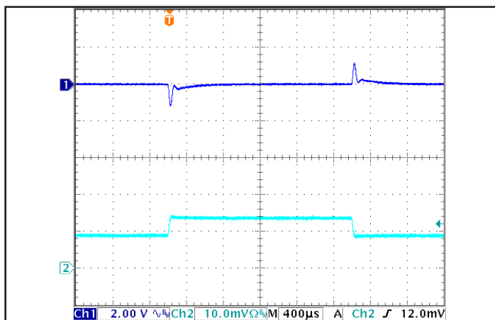
Figure 5: Output voltage response to step-change in load current (50%-75%-50% of I out (max); dI/dt = 0.1 A/μs). Load cap: 1 μF ceramic capacitor. Ch 1: V out (2 V/div), Ch 2: I out (5 A/div).
