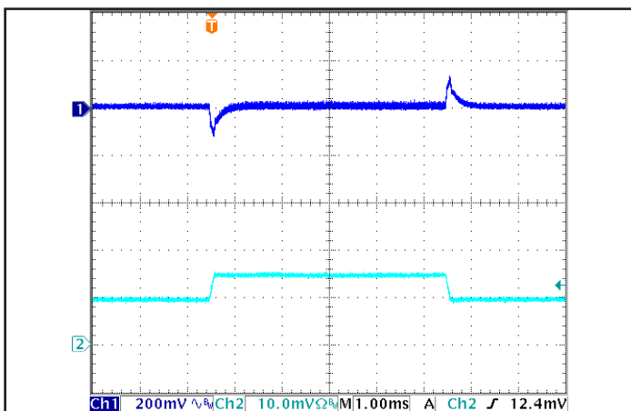
Figure 5: Output voltage response to step-change in load current (50%-75%-50% of Iout(max); dI/dt = 0.1 A/μs). Load cap: 1 μF ceramic and 15 μF tantalum capacitors. Ch 1: Vout (200 mV/div), Ch 2: Iout (20 A/div).
