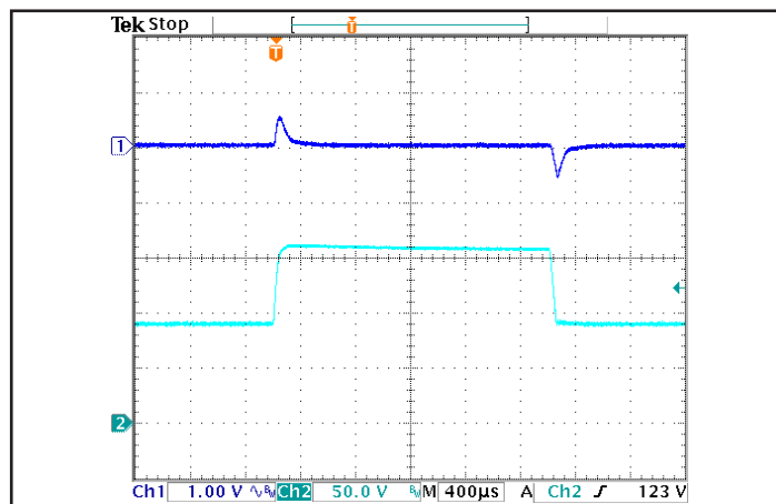
Figure 6: Output voltage response to step-change in input voltage (1000 V/ms). Load cap: 100 μF electrolytic output capacitance. Ch 1: V out (1 V/div), Ch 2: V in (50 V/div).
