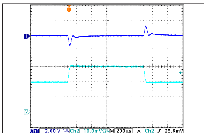
Figure 5: Output voltage response to step-change in load current (50%-75%-50% of I out (max); dI/dt = 0.1 A/μs). Load cap: 1 μF ceramic capacitor. Ch 1: V out (2 V/div), Ch 2: I out (2 A/div).
