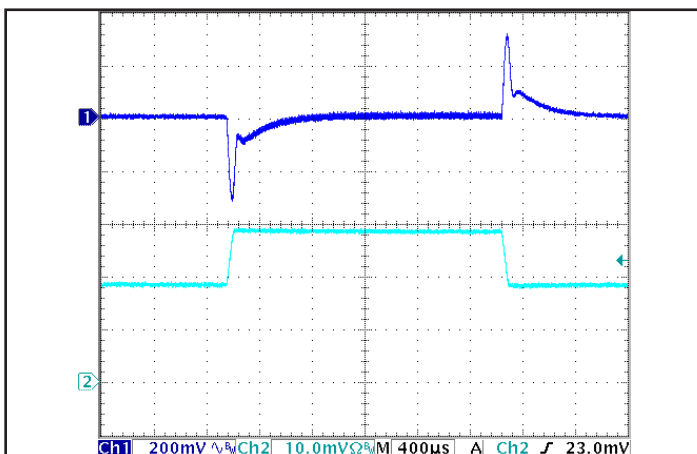
Figure 5: Output voltage response to step-change in load current (50%-75%-50% of I out (max); dI/dt = 0.1 A/μs). Load cap: 1 μF ceramic and 15 μF tantalum capacitors. Ch 1: V out (200 mV/div), Ch 2: I out (5 A/div).
