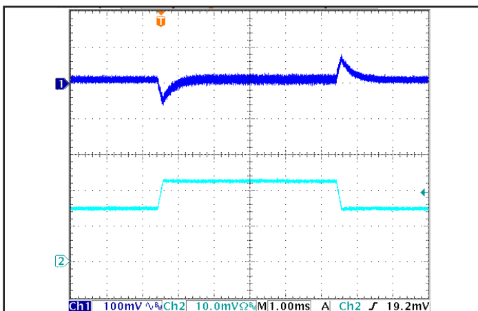
Figure 5: Output voltage response to step-change in load current (50%-75%-50% of Iout(max); dI/dt = 0.1 A/μs). Load cap: 1 μF ceramic and 15 μF tantalum capacitors. Ch 1: Vout (100 mV/div), Ch 2: Iout (20 A/div).
