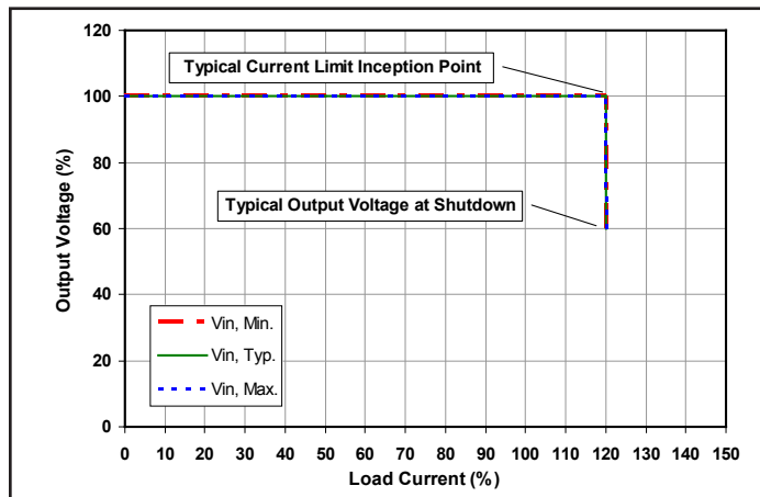
Common Figure 2: Output voltage vs. load current showing typical current limit inception points and converter shutdown points.
